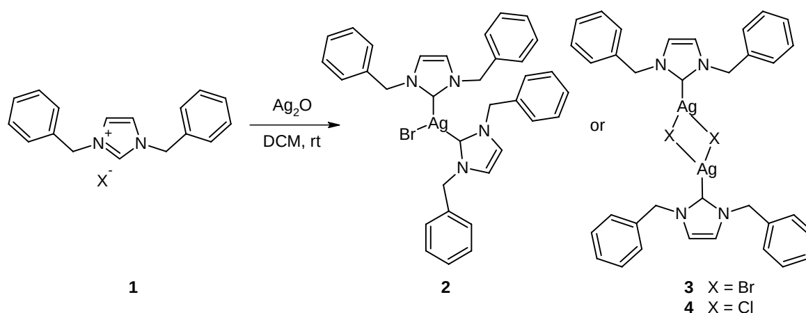
Scheme 2.1. Reaction of imidazolium halide with Ag_2O , yielding 2 or 3 ( 4 ).
