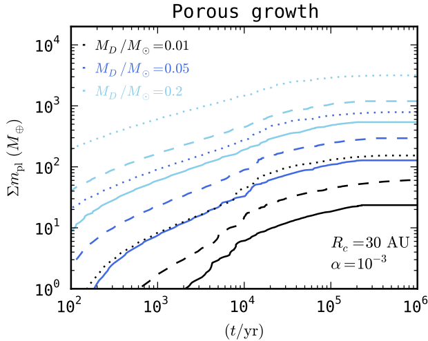
Figure 5.7: Total mass of planetesimals as a function of time for porous growth without erosion. Different linestyles indicate Z_0 = 0.01 (solid); Z_0 = 0.02 (dashed); and Z_0 = 0.05 (dotted). The total planetesimal mass increases significantly with disk mass and disk metallicity.
