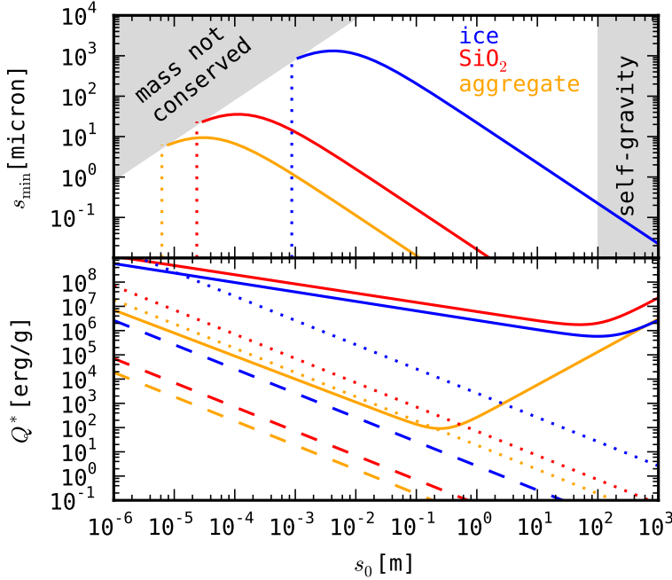
Figure 6.1: Top: Minimum fragment size s_{\min} in a 20 m/s collision (Eq. 6.4) for three materials, as a function of collider size s_0 . We have assumed \eta = 10^{-2} and s_{\max} = 2^{-1/3} s_0 . The grey shaded areas are excluded because of mass conservation (left), and self-gravity (right). The dotted lines indicate the limit of Eq. 6.6. Bottom: Critical energies versus size for equal-sized collisions. The energy needed to split a particle (e.g., Eq. 6.6) is shown for \eta = 10^{-3} (dotted) and \eta = 1 (dashed). The solid curves correspond to catastrophic fragmentation of aggregates (Beitz et al. 2011), and ice and basalt (Benz & Asphaug 1999), showing both the strength-dominated (small sizes) and self-gravity dominated regimes (large sizes).
