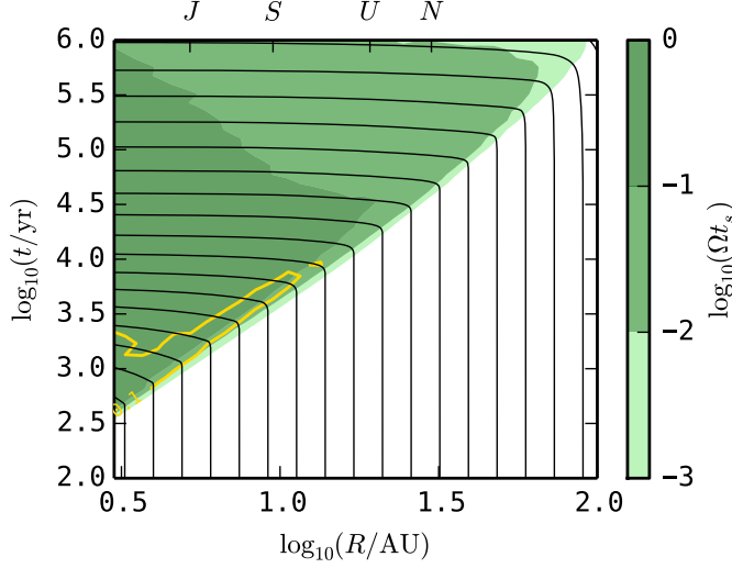
Figure 5.13: Dust evolution for porous growth followed by erosion, in a compact 0.01 M_{\odot} disk with \alpha = 10^{-3} and Z_0 = 0.02 (same model as Fig. 5.11). Times/locations where the mass-dominating particles have 10^{-3} \leq \Omega t_s \leq 1 have been colored green, and the contours depict (\rho_d^*/\rho_g)_{z=0} = \{0.1; 0.5; 1\} .
