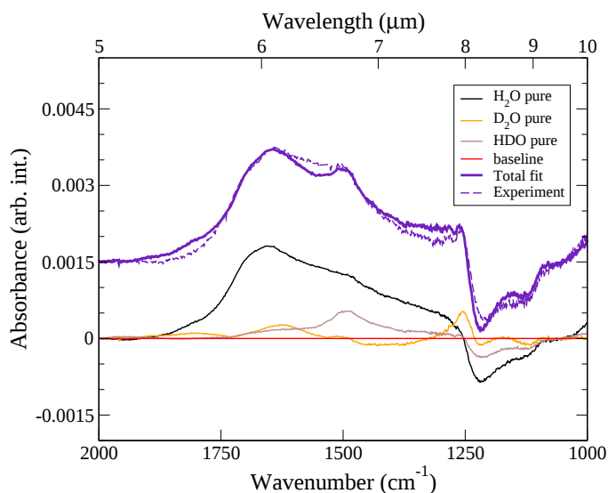
Figure 7.3: Example of a recorded spectrum in the water bending region (130 K) and its best fit, decomposed into the separate components ( \text{H}_2\text{O} , \text{HDO} , and \text{D}_2\text{O} - see Fig. 7.2), recorded after 210 minutes. Note: this concerns experiment 5 from Table 7.1. Pure spectra themselves compensate for the baseline artifact at 1200\text{ cm}^{-1} .
