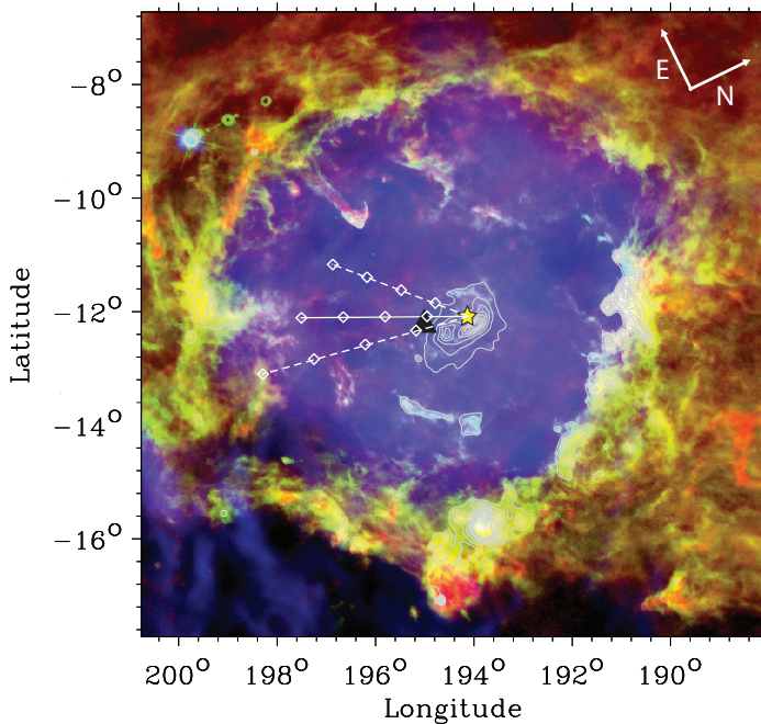
Figure 5.5: Three-color image of the \lambda Ori bubble. The color codes are the same as Fig. 5.1a. Overlaid are contours of IRAS 60\ \mu\text{m} , with intensity levels: 100% (maximum intensity) - 90% - 80% - 70% - 60% - 50% - 40% - 30%. The solid line marks the past trajectory of the star \lambda Ori during 4 Myr given its current space motion. Open diamond symbols mark intervals of 1 Myr. The dashed lines are the extremes of possible space motion considering the errors in proper motion and distance to the star. The black triangle marks the center of expansion of the \lambda Ori bubble (Lang & Mashedier 1998).
