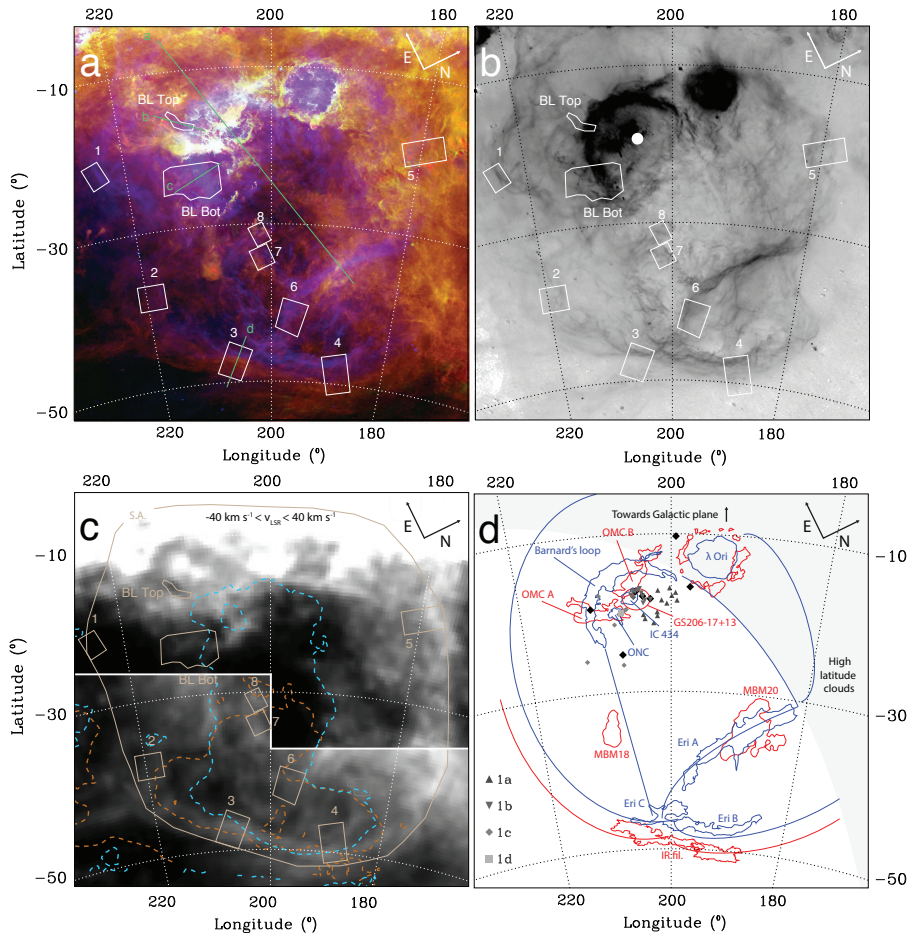
Figure 5.1: (a) Three-color image of the Orion-Eridanus superbubble. H \alpha (blue) reveals ionized gas, surrounded by a layer of PAHs or stochastically heated small grains, traced by the WISE 12 \mu m band (green). Red is Planck 353 GHz that probes cold (20 K) dust. The PAHs/small grains trace the UV-illuminated edges of clouds of cold dust so that red and green blend to form yellow. To the northeast lies the Galactic plane, while to the northwest lie high-latitude clouds (e.g., Schlafly et al. 2014). The numbered boxes define the apertures discussed in Sec. 5.3.2; the light-green solid lines are cross-cuts used in Fig. 5.2. (b) Same as panel (a), but only showing H \alpha emission. The white dot marks the flux-weighted center of the H \alpha bubble (Reynolds & Ogden 1979). (c) LAB -40 km s ^{-1} < v_{\text{LSR}} < 40 km s ^{-1} HI emission (Brown et al. 1995). Overlaid are contours of ROSAT 0.25 keV (orange dashed) and ROSAT 0.75 keV diffuse X-rays (light blue dashed). The 0.75 keV emission projected in Barnard’s Loop originates from the ONC and IC 434 regions, but is blended with diffuse emission from the superbubble. The white solid line marks a different scaling to accentuate the faint HI filament intersecting apertures 2-4. Also plotted is the shape of the superbubble aperture (S.A.; see text) (d) Schematic representation of the region. H \alpha gas structures are shown in blue lines/contours; dust structures are plotted in red. The solid lines trace faint filaments of the region to guide the eye in panels (a) & (b). Black diamonds are the stars that form the constellation of Orion. Members of Orion OB1 (Blaauw 1964; Brown et al. 1994) with spectral type B2 or earlier are shown in different grey symbols shown by the legend. See text for the different abbreviations.
