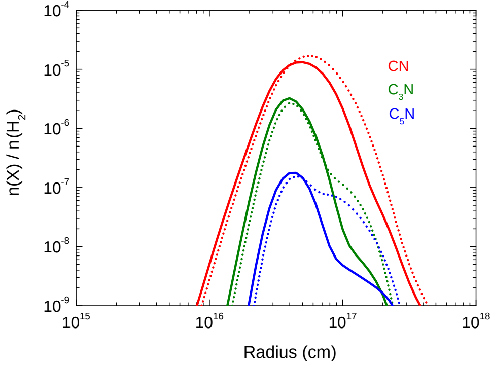
Figure 3.8 — Plot of the fractional abundances, relative to H_2 , of C_nN ( n=1, 3, 5 ) as functions of radii. Dotted and solid lines exhibit the results from the model of McElroy et al. (2013) and the SS model.
