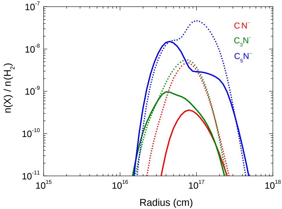
Figure 3.7 — Plot of the fractional abundances, relative to H_2 , of C_nN^- ( n=1, 3, 5 ) as a function of radius. Dotted lines: McElroy et al. (2013) model. Solid lines: SS model with updated shielding of N_2 and CO, details are described in Section 3.2.2.
