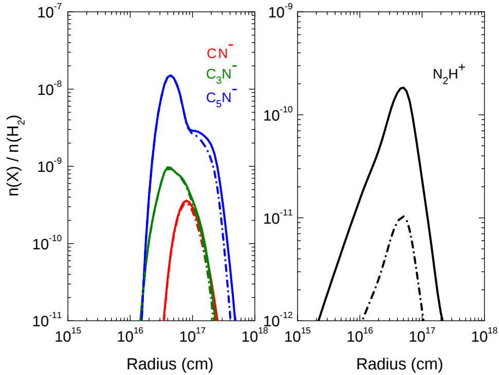
Figure 3.14 — Plot of the fractional abundances, relative to H_2 , of C_nN^- ( n = 1, 3, 5 ) (left panel) and N_2H^+ (right panel) as a function of radius. Solid lines: calculated using an initial N_2 abundance of 2 \times 10^{-4} (relative to H_2 ). Dash-dotted lines: calculated using an initial N_2 abundance of 1 \times 10^{-5} . In both cases, the SS model with updated shielding was employed.
