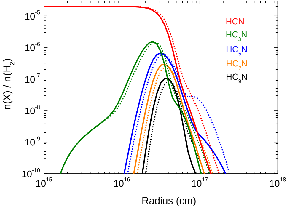
Figure 3.10 — Plot of the fractional abundances, relative to H_2 , of HC_nN ( n=1, 3, 5, 7, 9 ) as a function of radius from the center of the star towards the outside of the envelope. Dotted and solid lines exhibit the results from the model of McElroy et al. (2013) and the SS model.
