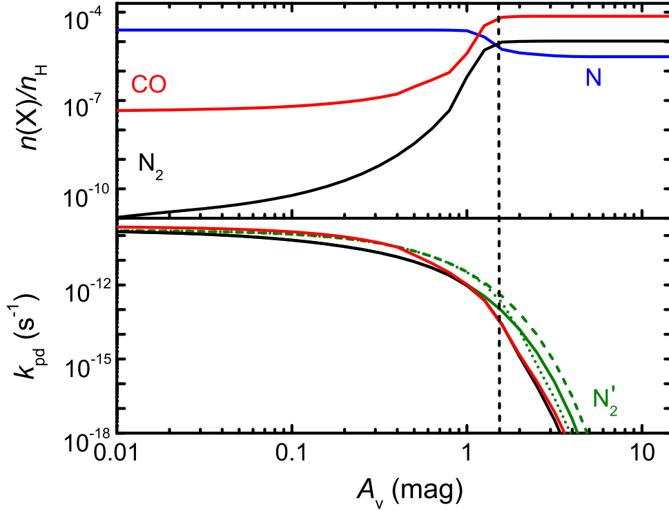
Figure 2.10 — Top: Relative abundances of N, N_2 and CO as a function of depth into a translucent cloud with \chi = 1 , T = 30 K and n_H = 10^3 \text{ cm}^{-3} . Bottom: Photodissociation rates of N_2 (black) and CO (red) as functions of depth. Alternative photodissociation rate curves ( N'_2 , green) consider shielding by dust alone (dashed), dust + self-shielding (dotted), and dust + H + H_2 (solid). The conversion from N to N_2 occurs at A_V \simeq 1.5 mag, as shown by the vertical dashed line.
