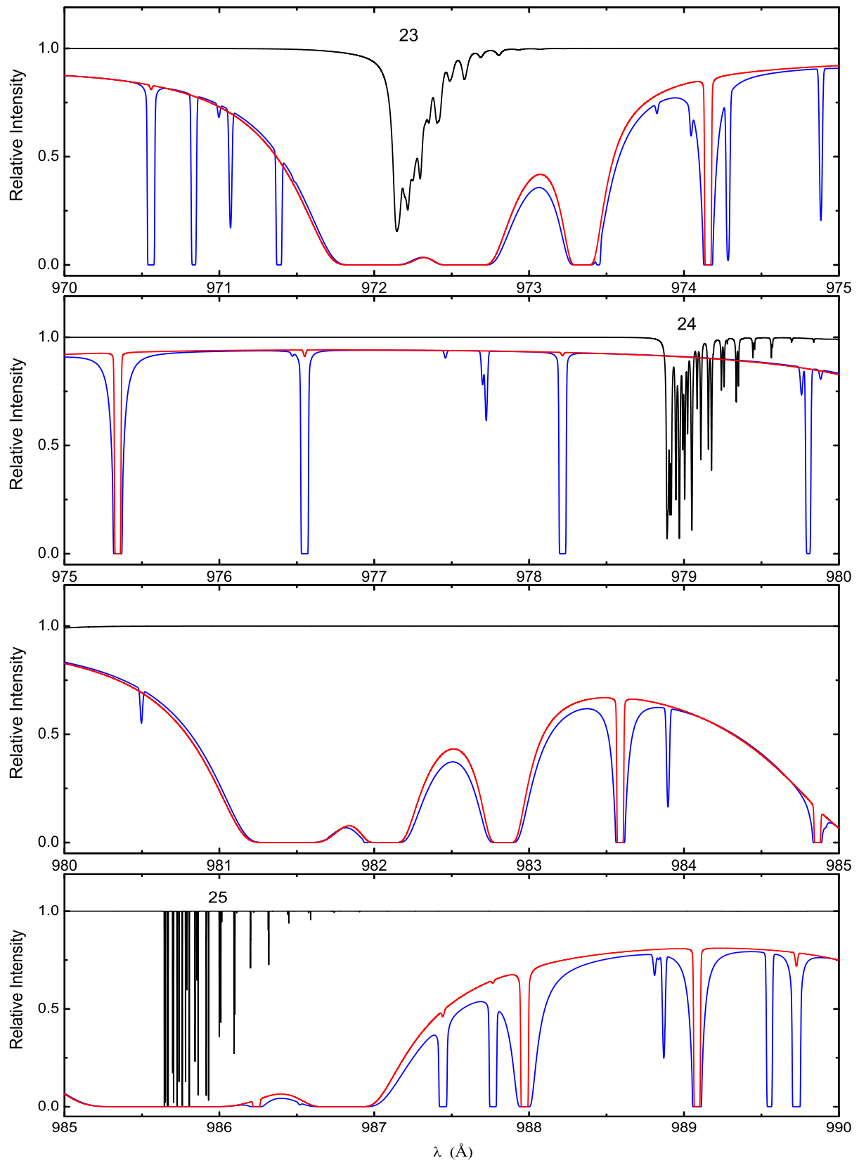
Figure 2.4 — As Fig. 2.1, but for 970–990 Å
