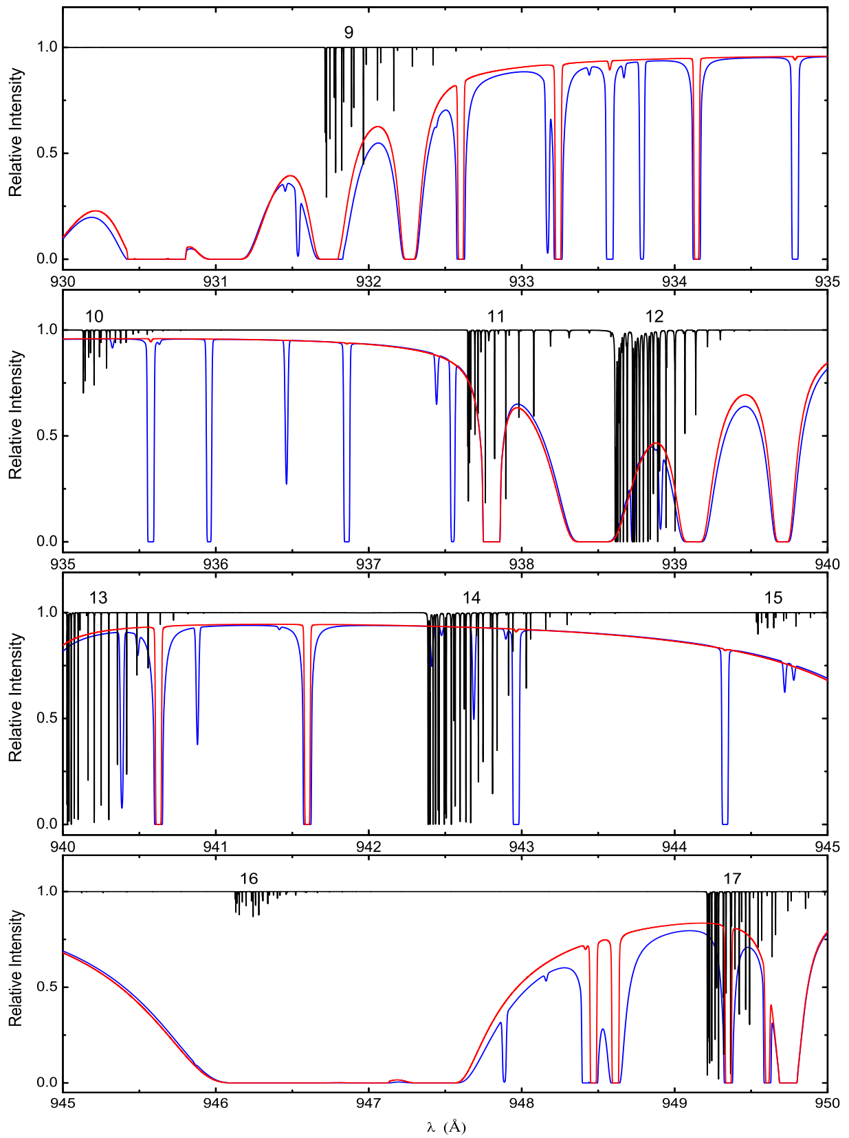
Figure 2.2 — As Fig. 2.1, but for 930–950 Å.
