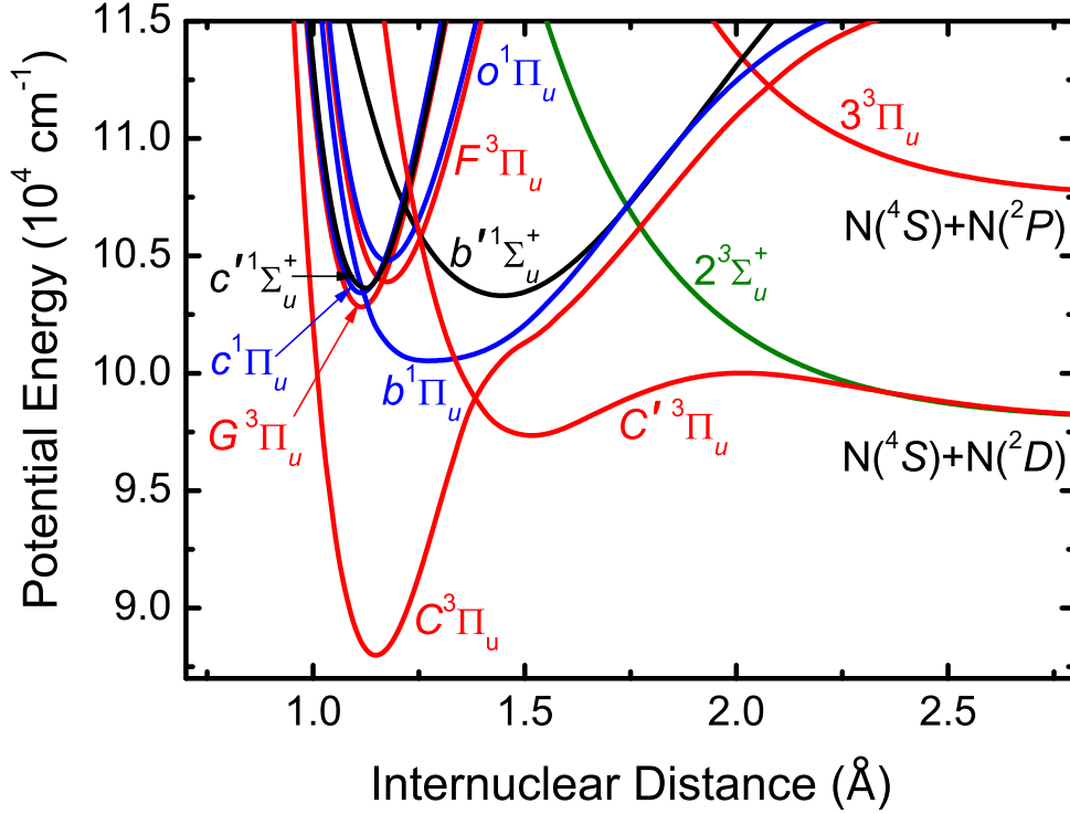
Figure 2.1 — Diabatic-basis potential-energy curves for electronic states of N_2 relevant to interstellar photodissociation. Blue curves: ^1\Pi_u states. Black curves: ^1\Sigma_u^+ states. Red curves: ^3\Pi_u states. Green curve: 2^3\Sigma_u^+ state. The energy scale is referenced to the v=0, J=0 level of the X^1\Sigma_g^+ ground state (not shown). The lowest dissociation limit, N(^4S)+N(^4S) at \sim 78\,715\text{ cm}^{-1} (9.76 eV), is beyond the scale of the figure. The H ionization potential of 13.6 eV provides an upper limit to the interstellar radiation field and corresponds to 109\,691\text{ cm}^{-1} .
