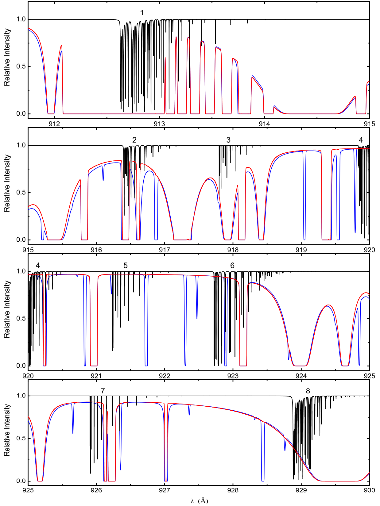
Figure 2.1 — Zoom-in of the high-resolution spectra of \text{N}_2 (black line) and \text{H} plus \text{H}_2 (red line) in the wavelength range of 911.75–930 Å for a thermal excitation temperature of 50 K. The column density of \text{N}_2 is 10^{15} \text{ cm}^{-2} and values for \text{H}_2 and \text{H} are taken to be half of the observed column densities in the well-studied diffuse cloud toward \zeta Oph, as is appropriate for the center of the cloud: N(\text{H}_2)=2.1 \times 10^{20} and N(\text{H})=2.6 \times 10^{20} \text{ cm}^{-2} . The model \text{H}_2 Doppler width is 3 \text{ km s}^{-1} . Also shown is the \text{H}_2 + \text{H} absorption spectrum (blue) towards \zeta Oph using the observed column densities for individual J levels, showing non-thermal excitation of \text{H}_2 .
