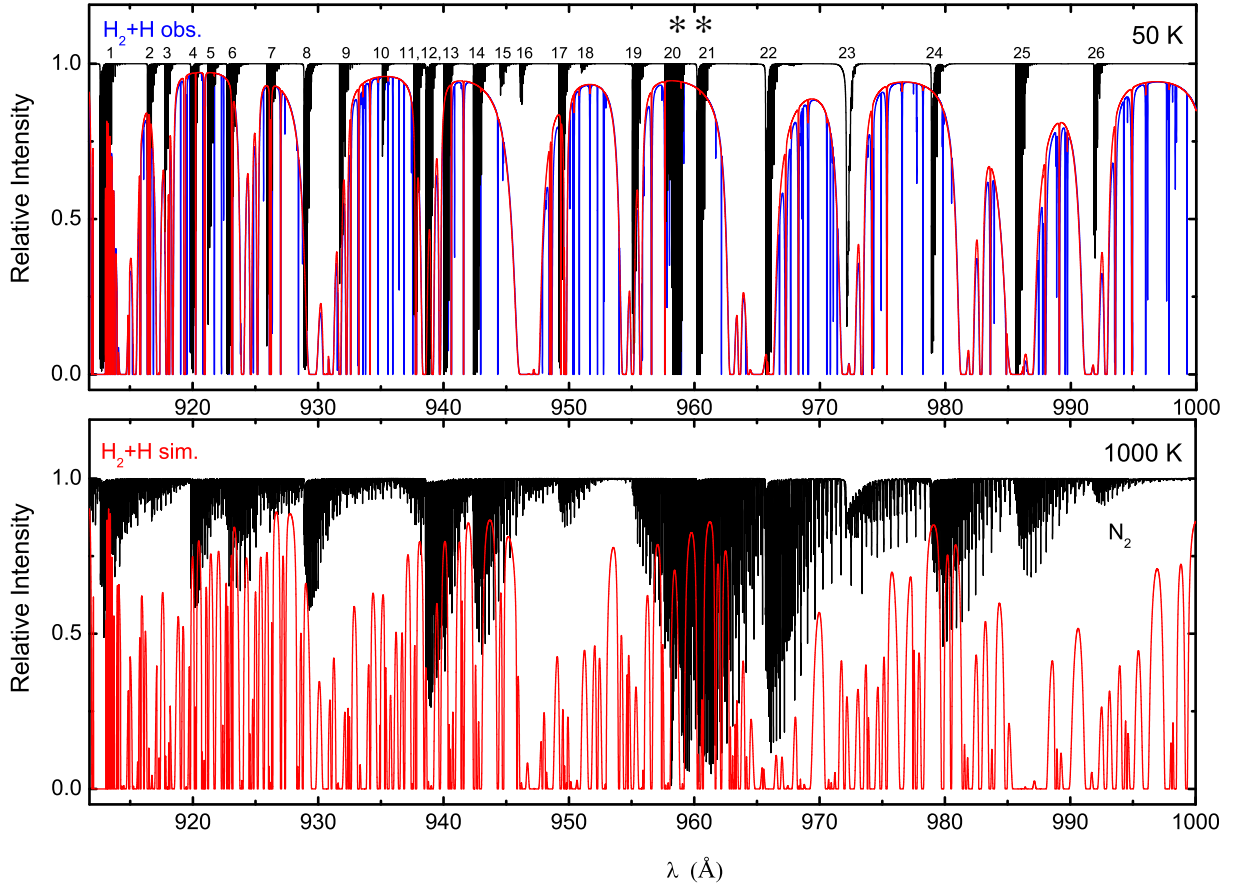
Figure 2.4 — Simulated absorption spectra for N_2 (black) and H_2 + H (red) in the wavelength range 912–1000 \text{\AA} assuming thermal excitation temperatures of 50 (top) and 1000 K (bottom). The column density of N_2 is 10^{15} \text{ cm}^{-2} and values for H_2 and H are taken to be half of the observed column densities in the well-studied diffuse cloud toward \zeta Oph, as is appropriate for the center of the cloud: N(H_2)=2.1 \times 10^{20} and N(H)=2.6 \times 10^{20} \text{ cm}^{-2} . The model H_2 Doppler width is 3 \text{ km s}^{-1} . Also shown is the H_2 + H absorption spectrum (blue) towards \zeta Oph using the observed column densities for individual J levels, showing enhanced non-thermal excitation of H_2 in the higher J levels. The asterisks indicate the c'(0) (Band 20) and c(0) (Band 21) bands, respectively, detected in absorption towards HD 124314.
