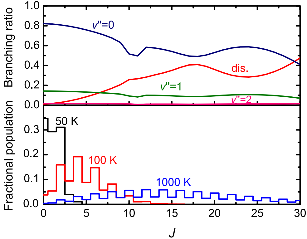
Figure 2.2 — Top: The branching to various decay channels of the c'(v' = 0) excited-state of N_2 as a function of total rotational quantum number, J . The figure includes spontaneous emission to several non-dissociative ground state vibrational levels ( v'' = 0, 1 and 2 ) and decay due to predissociation ( dis. ). Bottom: Fractional population of the N_2 ground state in its lowest vibrational level as a function of J and for several excitation temperatures. The 2:1 ratio of populations for even:odd J levels arises from the combined rotational and nuclear spin statistics.
