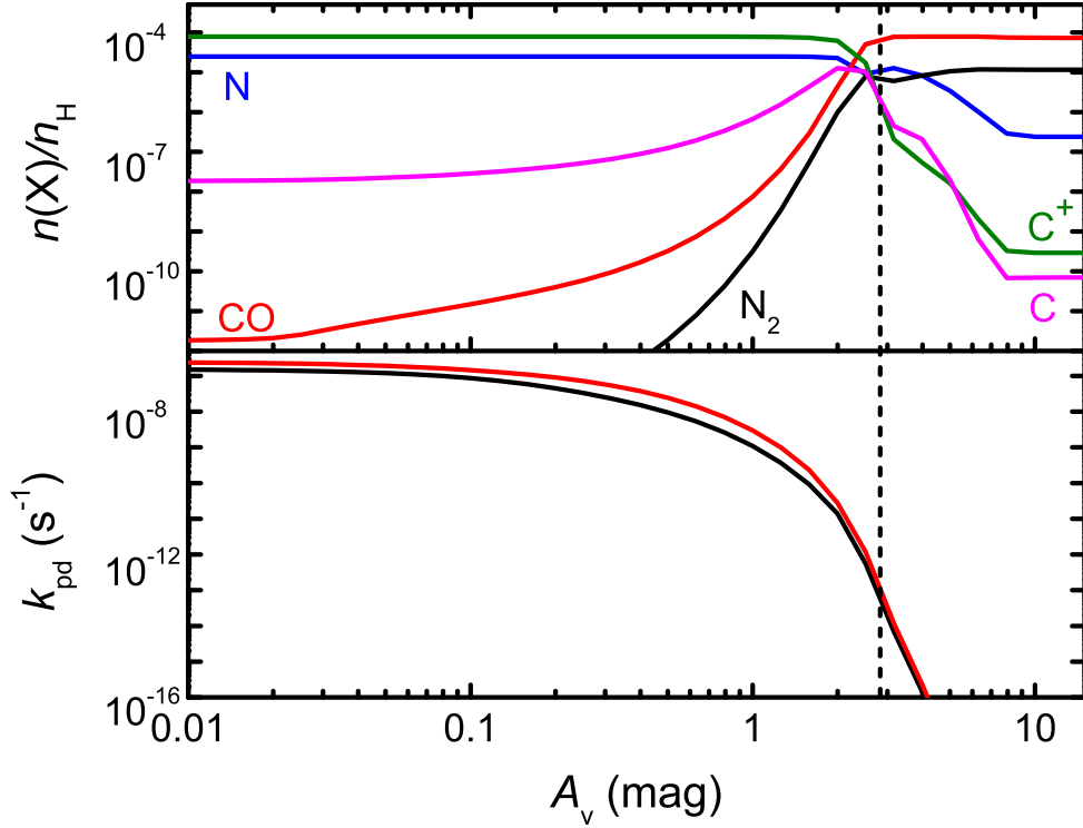
Figure 2.12 — Top: Relative abundances of N (blue), N_2 (black), C (magenta), C^+ (green) and CO (red) as functions of depth into a dense PDR. Bottom: Photodissociation rates of N_2 and CO as functions of depth into a dense PDR. The vertical dashed line indicates where He^+ and H_3^+ take over from photodissociation as the main destruction mechanism for N_2 .
