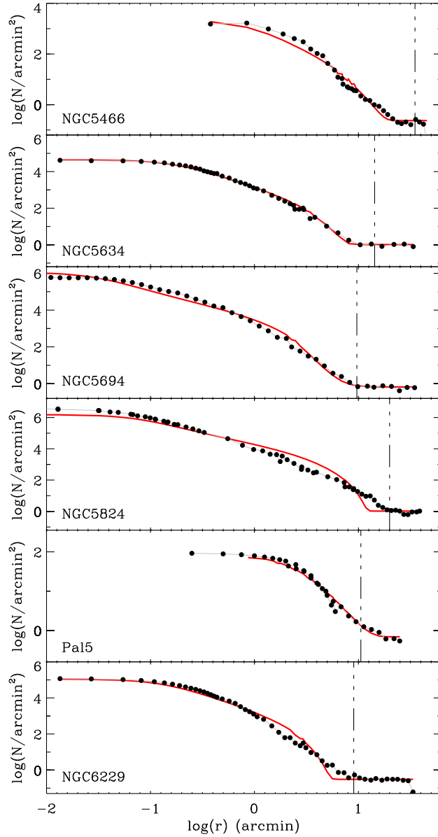
Figure 5.5: Radial density profiles as derived by for NGC 5466, NGC 5634, NGC 5694, NGC 5824, Pal 5 and NGC 6229. The vertical line indicate the distances from the cluster centre where the cluster content has been separated from the rest of objects in the photometric catalogues. The red line corresponds with the best King model fitting (Carballo-Bello et al. 2012).
