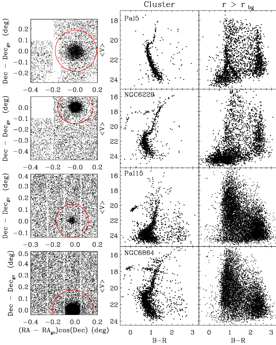
Figure 5.14: CMDs corresponding to the clusters Pal 5, NGC 6229, Pal 15 and NGC 6864 (middle column) and to those objects beyond r_{bg} from the cluster centre (right column). A map showing the distribution of the stars in the catalog with respect to the cluster centre is also included (left), where r_{bg} is indicated by a red line.
