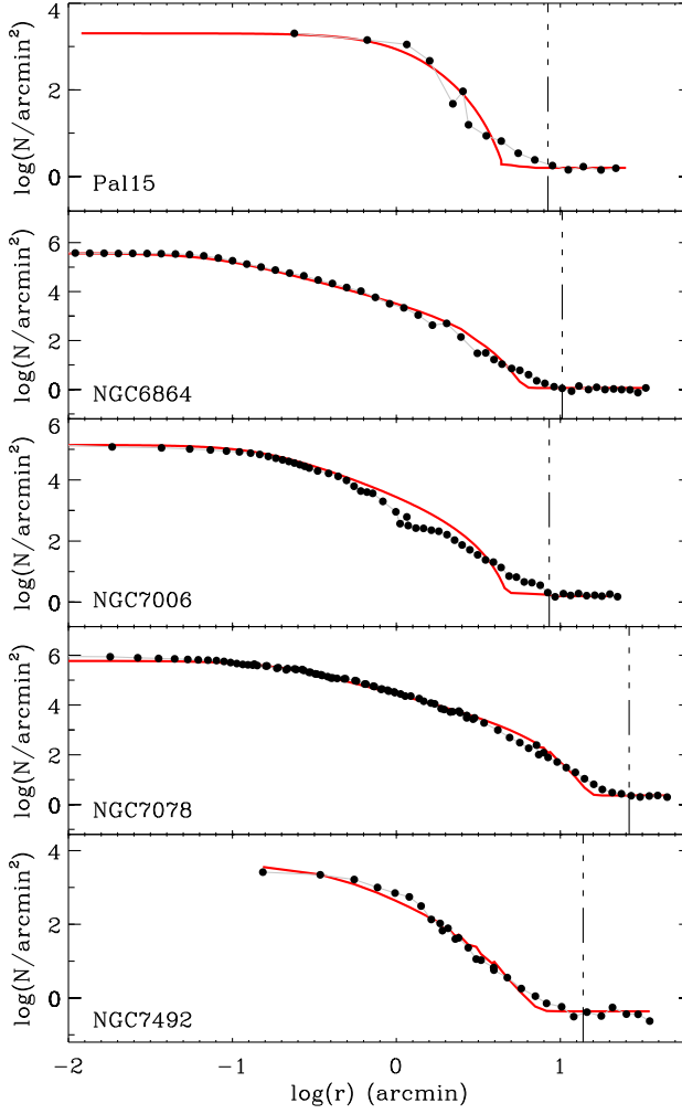
Figure 5.6: Radial density profiles as derived by for Pal15, NGC 6864, NGC 7006, NGC 7078 and NGC 7492. The vertical line indicate the distances from the cluster centre where the cluster content has been separated from the rest of objects in the photometric catalogues. The red line corresponds with the best King model fitting (Carballo-Bello et al. 2012).
