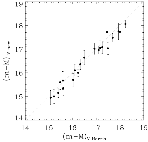
Figure 5.9: Comparison between the Harris (2010) distance moduli and the values derived using the isochrone fitting method described in Section 5.3.4. (m-M)_V and (m-M)_{V \text{ Harris}} represent the distance modulus obtained for the GCs included in our sample and the one taken from the Harris catalog respectively. The dashed line indicates the 1:1 relation.
