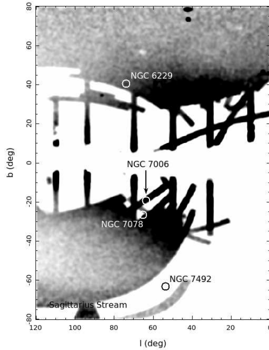
Figure 5.19: Density maps generated from SDSS data of the sky area where the GCs NGC 6229, NGC 7006, NGC 7078 and NGC 7492 are located. The huge stellar over-density observed might be associated whether with the Hercules-Aquila cloud (Belokurov et al. 2007a; Simion et al. 2014) or with the region of higher density of halo stars reported by Deason et al. (2014). Note the presence of the Sgr stream in the bottom left corner of the map.
