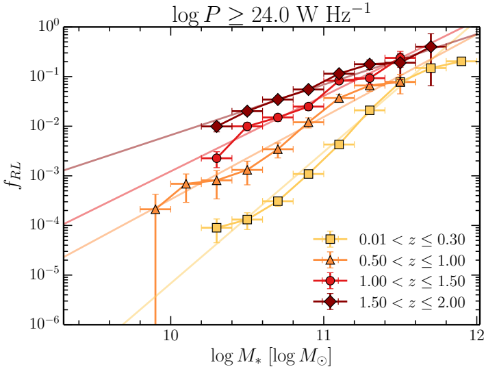
Figure 5.6: The fraction of galaxies hosting a radio source (radio-loud fraction) for a radio-power cut-off of P_{1.4\text{GHz}} > 10^{24} \text{ W Hz}^{-1} in the four redshift bins. The coloured lines show a linear fit over the stellar mass range 10 < \log(M_*/M_\odot) < 11.5 . The slopes of these fits are 2.7 \pm 0.2 , 1.7 \pm 0.2 , 1.5 \pm 0.1 and 1.0 \pm 0.1 from the lowest to highest redshift bins.
