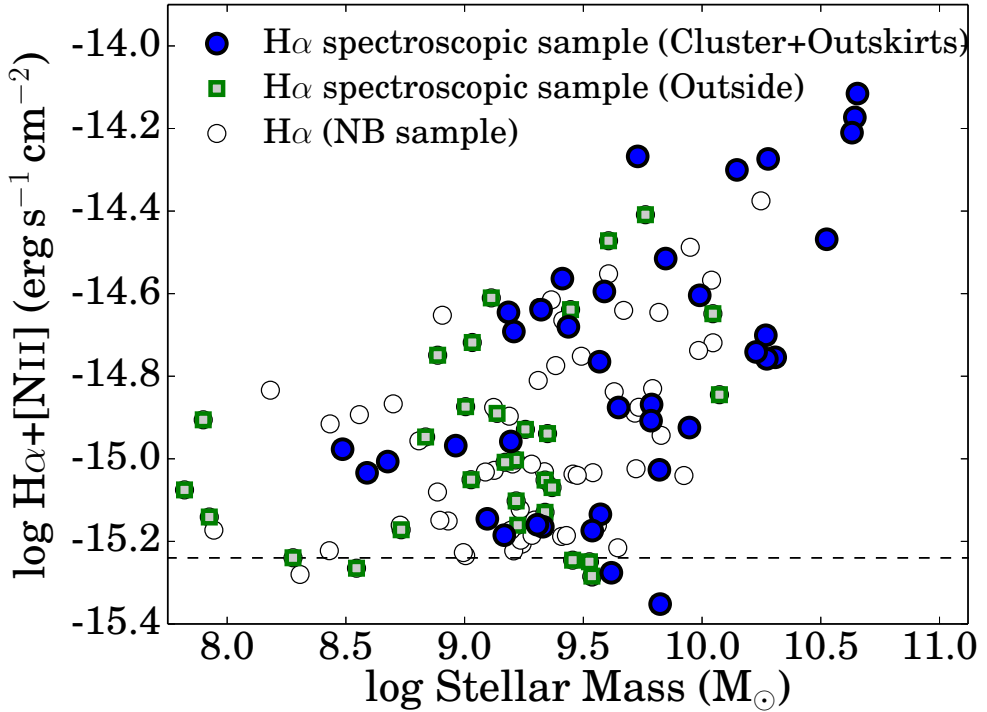
Figure 8.7: The relation between H\alpha + [\text{NII}] flux (corrected for Galactic extinction, but not corrected for intrinsic dust extinction), based on 5'' narrow-band photometry and stellar mass, for the parent sample, selected using narrow-band, and our spectroscopic sample. Our spectroscopically confirmed sources sample the vast majority of the parameter space, both for galaxies in the cluster ( R < 1.5 Mpc) and outskirts ( 1.5 < R < 2.5 Mpc) and for those outside the cluster. We are particularly complete, relative to the parent sample, for stellar masses > 10^9 M_{\odot} . We preferentially miss sources with the lowest fluxes and with stellar masses lower than \sim 10^9 M_{\odot} .
