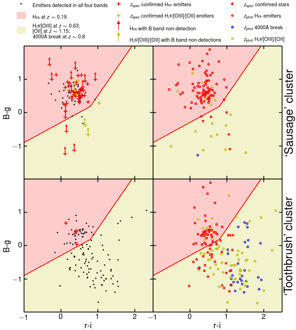
Figure 7.5: Colour-colour plot of ‘Sausage’ (top) plot and ‘Toothbrush’ (bottom plot) emitters, selected according to the criteria described in Fig. 7.4. B - g versus r - i colours are plotted. H\alpha emitters are expected to lie above and to the left of the thick red lines, in the red shaded areas. H\beta , [OIII] , [OII] emitters and 4000\text{\AA} break galaxies lie in the yellow shaded area. Left panels: Sources with clear detections are plotted with black dots. Spectroscopically confirmed H\alpha emitters are plotted in red crosses. Right panel: Sources with photometric redshifts consistent with being H\alpha emitters at z \sim 0.2 are plotted with red circles. Possible 4000\text{\AA} break galaxies are plotted in blue. Sources with photo- z ’s around 0.63 (between 0.5 and 0.7) and 1.15 (between 1.0 and 1.2) are selected as H\beta , [OIII] and [OII] emitters (plotted in yellow).
