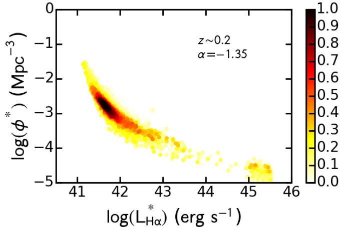
Figure 10.9: The values of LF Schechter parameters \phi^* and L_{\text{H}\alpha}^* , when we fix \alpha = -1.35 . For fitting the LF, we create 1000 random sub-samples of H \alpha emitters, at a range of probed volumes. The data points are colour coded with the co-moving volume probed in units of 1000 \text{Mpc}^3 . Note how at small volumes the scatter is the value is extremely large (up to 4 – 5 dex), while at large volumes the values for \phi^* and L_{\text{H}\alpha}^* converge. We obtain similar results with a different value of \alpha or when we use the data for the two filters separately (see Figure 10.16)
