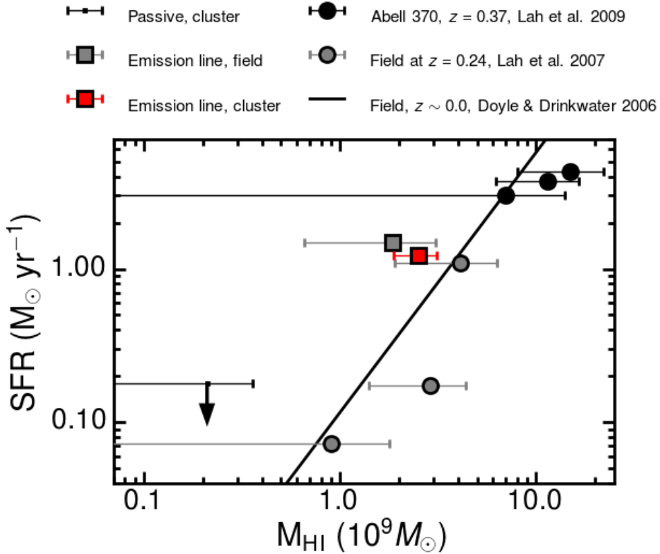
Figure 9.8: Relationship between SFR and integrated HI mass. All SFRs are calculated with a Chabrier IMF. For the passive population, the SFR is an upper limit. Overplotted are the data points for cluster Abell 370 at z = 0.37 (Lah et al. 2009) and a blank field at z = 0.24 (Lah et al. 2007), together with the SFR- M_{\text{HI}} relationship for the local Universe (Doyle & Drinkwater 2006). Note that it is difficult to compare our dataset with other work because of the different ways of measuring the HI mass and the different SF tracers used ( \text{H}\alpha , [OII] or IR).
