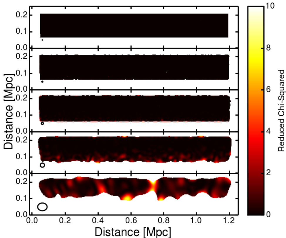
Figure 3.6: \chi^2 maps associated to the JP spectral ageing fits to the simulated data. The data are in order of ascending beam size from top to bottom: 1^2 , 2^2 , 4^2 , 8^2 , 18.0 \times 14.8 arcsec. The beam is shown in the bottom-left corner of each image.
