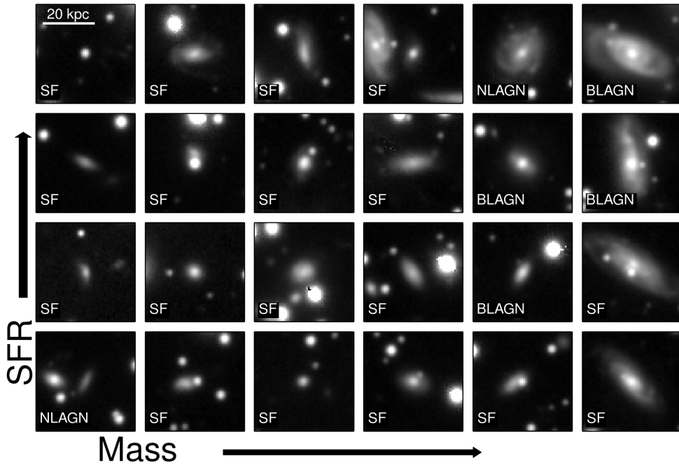
Figure 8.11: Thumbnails of our H\alpha cluster members. Each square is \sim 40 \times 40 kpc and we organise galaxies in respect to their estimated stellar mass and estimated star-formation rate. We also indicate which sources are likely AGN and which are star-forming. We do not find any evidence for significant galaxy-galaxy (major) merging. This implies that the enhanced star-formation and AGN activity within the merging cluster is not being driven by galaxy-galaxy mergers, and thus is it more likely driven by the interaction with the environment, and in particular with the shock wave. We note that the bright point sources, which show up in most images are stars within the Milky Way, not galaxies.
