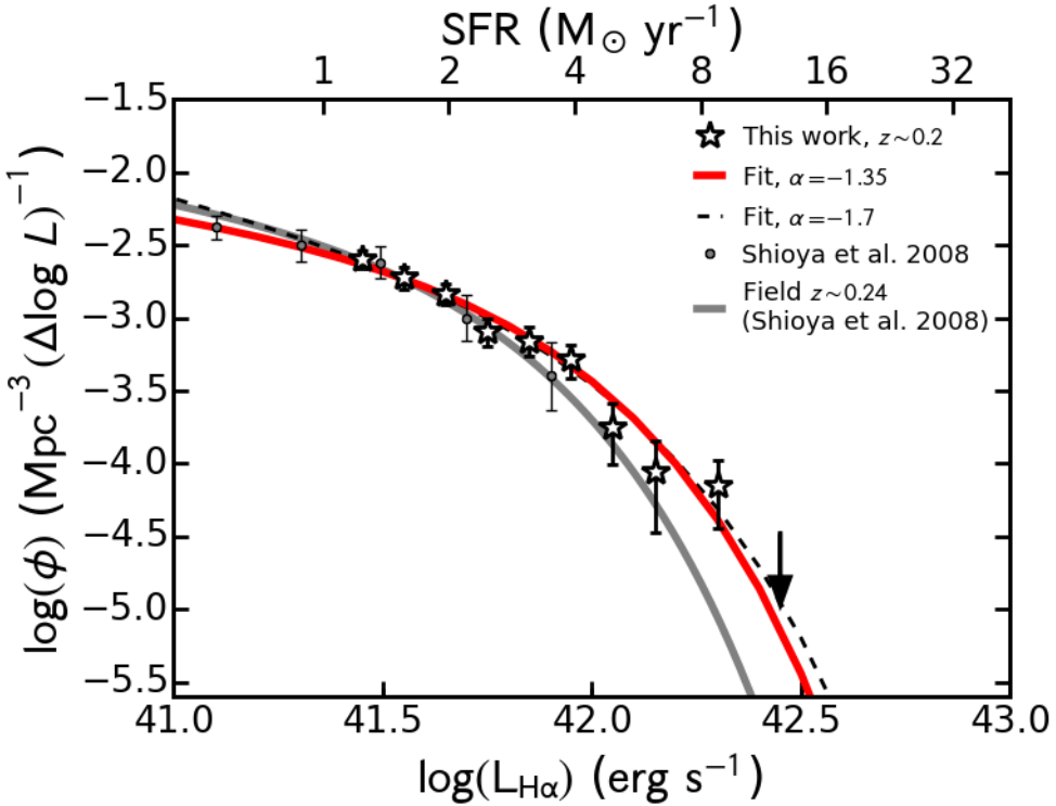
Figure 10.5: The H \alpha luminosity function at z \sim 0.2 from our study and the best fit Schechter function. The L_{H\alpha} is not corrected for intrinsic dust attenuation. For comparison, the results from Shioya et al. (2008) are also shown. Note the excellent agreement between the data in the overlapping luminosity range. However, our data probes brighter luminosities, enabling the first determination of the bright end of the H \alpha luminosity function at z \sim 0.2 .
