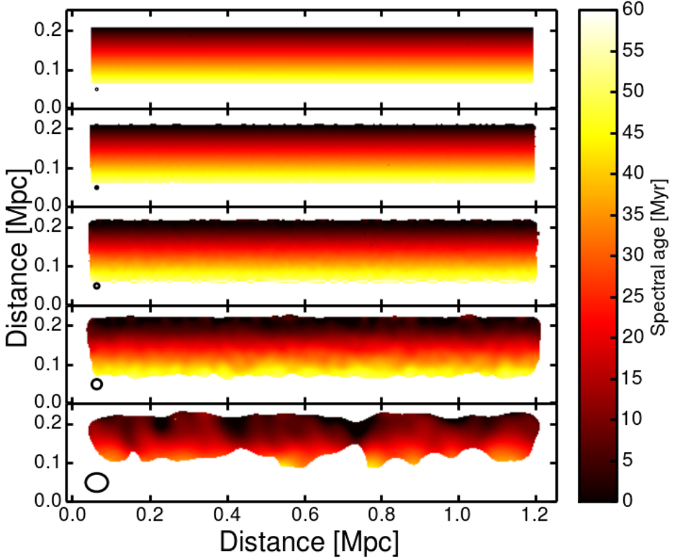
Figure 3.5: JP spectral ageing maps for the simulated data. The data are in order of ascending beam size from top to bottom: 1'' , 2'' , 4'' , 8'' , 18.0 \times 14.8 arcsec. The beam is shown in the bottom-left corner of each image.
