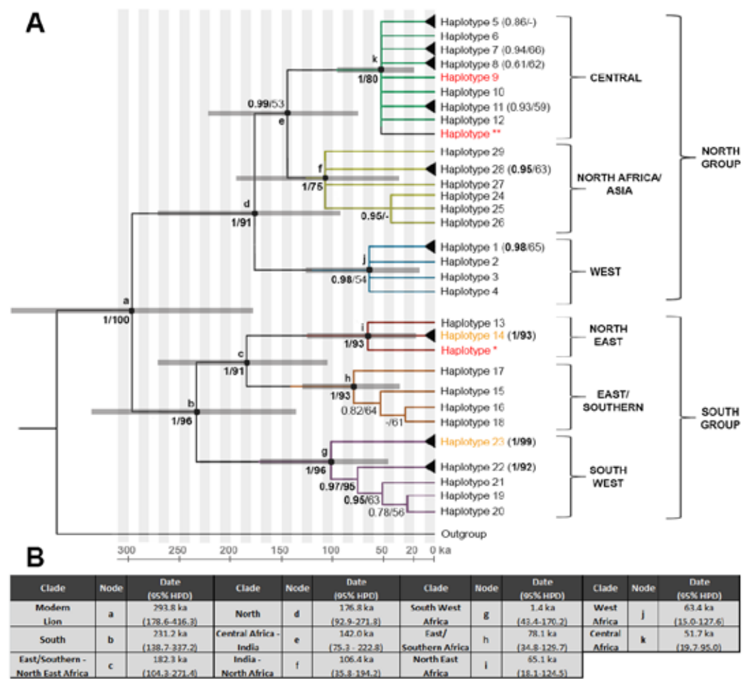
Supplemental Figure 2-1. Phylogenetic analyses for the complete lion dataset, including sixteen mitochondrial genomes and 178 cytb+ctrl reg. sequences. A: Phylogenetic tree of lion populations throughout their complete geographic range, based on complete mitochondrial genomes and cytb+ctrl reg. sequences. Branch colours correspond to haplotype colours in Supplemental Figure 2-2. Populations mentioned above as long branches with missing intermediate haplotypes, are indicated in orange. Populations with limited information regarding their origin, which were excluded from analyses presented in the main text, are shown in red. Support is indicated as posterior probability (Bayesian analysis)/bootstrap support (ML analysis). Branches with a single haplotype have been collapsed to improve readability. Support for these branches is indicated by a black triangle at the tip of the branch (support shown in the label). Nodes which have been included for divergence time estimates are indicated with letters and 95% HPD node bars. Distance to outgroup and nodes without dated split is not in proportion to divergence time. B: divergence time estimates and 95% HPD from BEAST analysis, also indicated as error bars in Supplemental Figure 2-1A.
