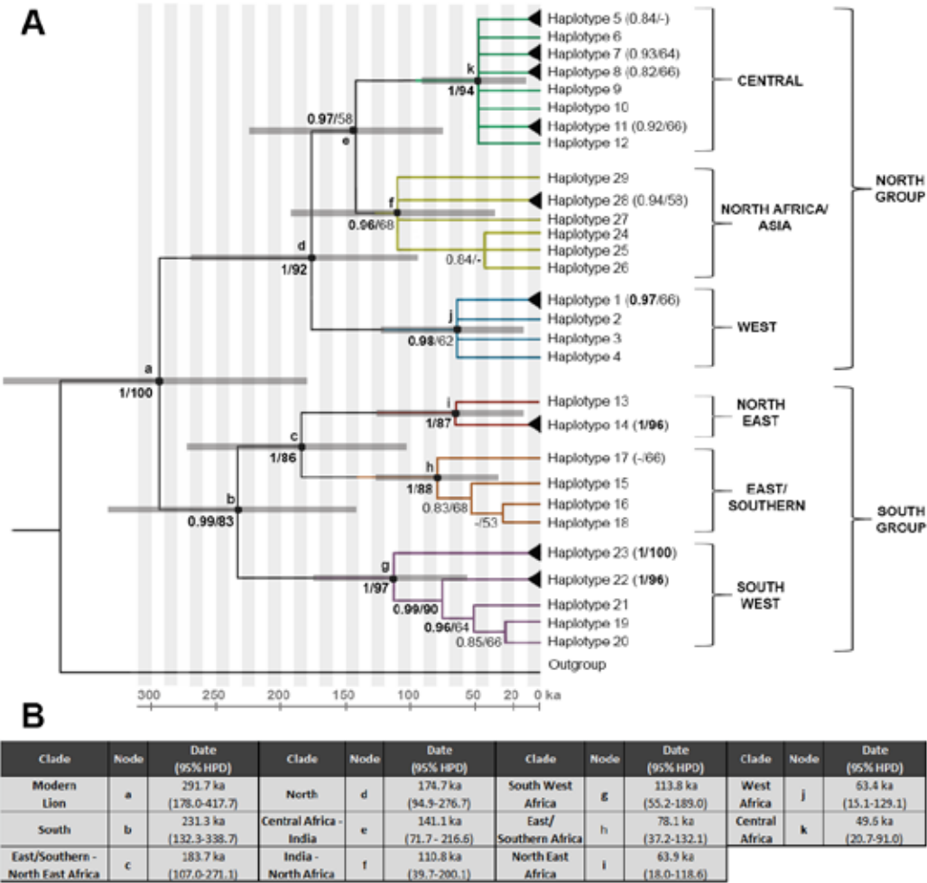
Figure 3. Phylogenetic analyses for the complete lion dataset, including sixteen mitochondrial genomes and 175 cytB + ctrl reg. sequences. A: Phylogenetic tree of lion populations throughout their complete geographic range, based on complete mitochondrial genomes and cytB + ctrl reg. sequences. Branch colours correspond to haplotype colours in Figure 4. Support is indicated as posterior probability (Bayesian analysis)/bootstrap support (ML analysis). Branches with a single haplotype have been collapsed to improve readability. Support for these branches is indicated by a black triangle at the tip of the branch (support shown in the label). Nodes which have been included for divergence time estimates are indicated with letters and 95% HPD node bars. Distance to outgroup and nodes without dated split is not in proportion to divergence time. B: divergence estimates and 95% HPD from BEAST analysis, also indicated as error bars in Figure 3A.
