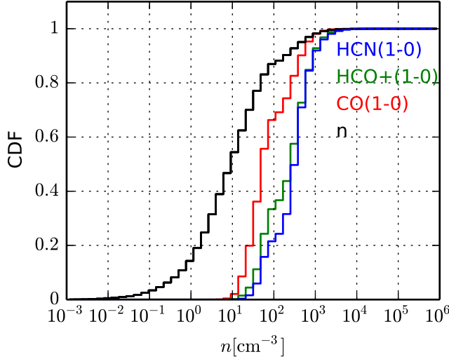
Figure 5.6 – Cumulative distribution of the densities and the luminosities of CO(1-0), HCO + (1-0) and HCN(1-0). For example, ~ 90% of the gas particles have a density n < 10^2 \text{ cm}^{-3} , whereas 75%, 40%, 20% of the emission of CO(1-0), HCO + (1-0) and HCN(1-0) emanate from gas whose density is lower than 10^2 \text{ cm}^{-3} .
