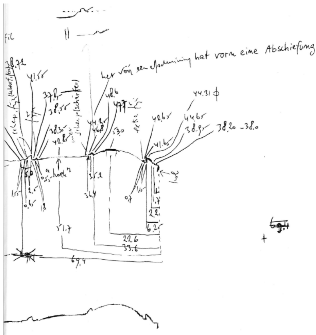
Figure 169. Measurements and drawings of 1135, D.I.E.u., Musikinstrumenten-Museum der Universität Leipzig, kindly provided by Stephan Blezinger.
