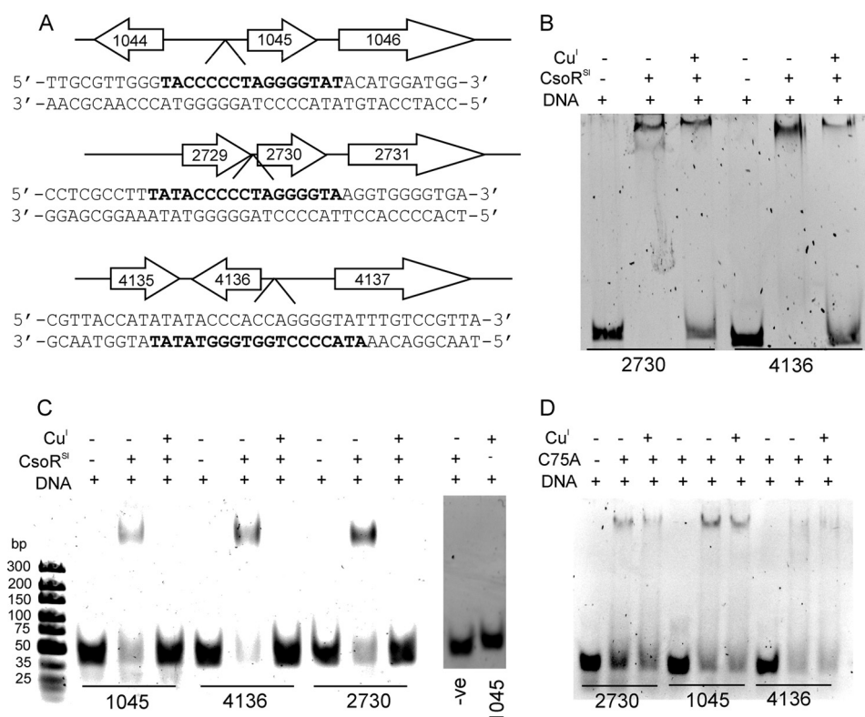
FIGURE 6. CsoR SL operator DNA targets and EMSA studies. A, three-locus regulon and the DNA sequences identified by PREDetector ( bold ) to be target operator binding sites for CsoR SL . The position of the DNA target sequence in the oligomers used in EMSA is highlighted in bold . B, EMSA of CsoR SL in the presence of the intergenic DNA fragments containing the target sequences for 2730 (232 bp) and 4136 (208 bp). C, EMSA of CsoR SL in the presence of the individual DNA oligomers containing the target sequences shown in A. The gel image to the right is a control EMSA showing the effect on binding CsoR SL to a randomly generated double-stranded DNA oligomer with the sequence 5'-GACGAGGACGTCTACGCCATCGACATACTG-3' and the mobility of the 1045 DNA oligomer in the presence of only Cu(I). D, EMSA of the C75A mutant of CsoR SL in the presence of the individual DNA oligomers containing the target sequences shown in A. The components present in each lane of the gel image are indicated with 0.5 \mu M [DNA] and 5 \mu M [apo-CsoR SL monomer] and [Cu I -CsoR SL monomer] used.
