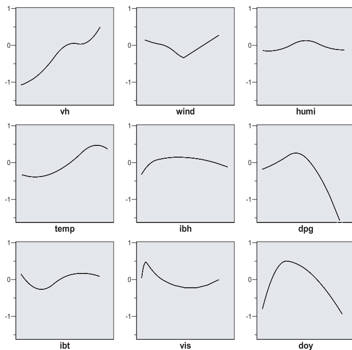
Figure 3.2. CATREG nonmonotonic spline transformations for the ozone data. The y-axis represent the quantifications multiplied with the regression coefficient for the predictor.
