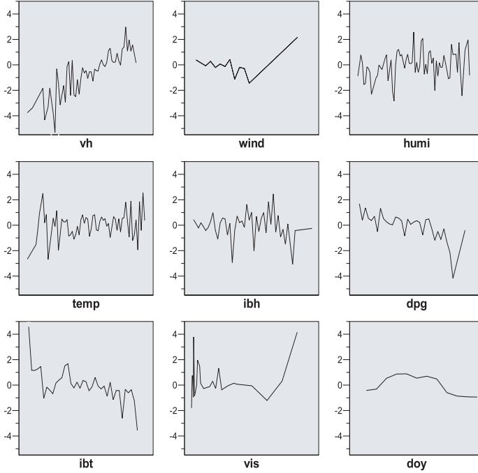
Figure 3.4. CATREG nominal transformations for the recoded ozone data. The y-axis represent the quantifications multiplied with the regression coefficient for the predictor.
