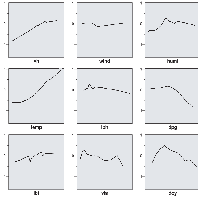
Figure 3.3. ACE supersmoothing transformations for the recoded ozone data.
