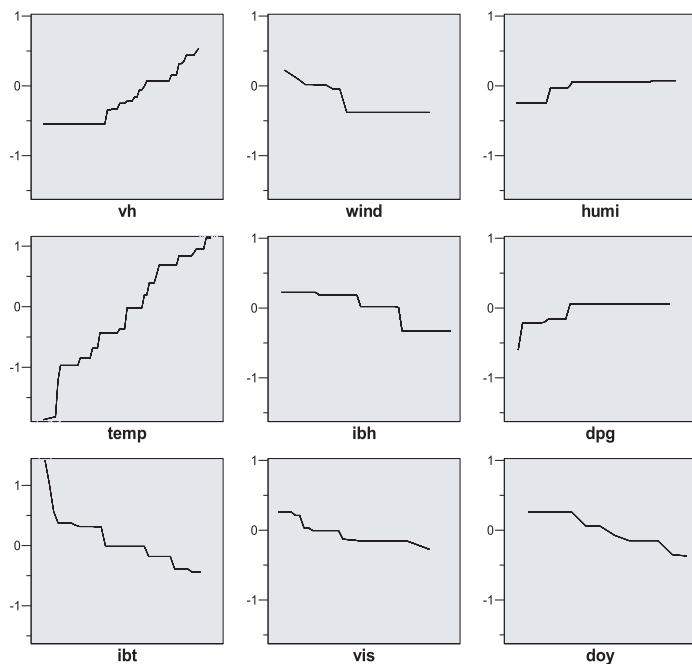
Figure 3.5. CATREG ordinal transformations for the recoded ozone data. The y-axis represent the quantifications multiplied with the regression coefficient for the predictor.
