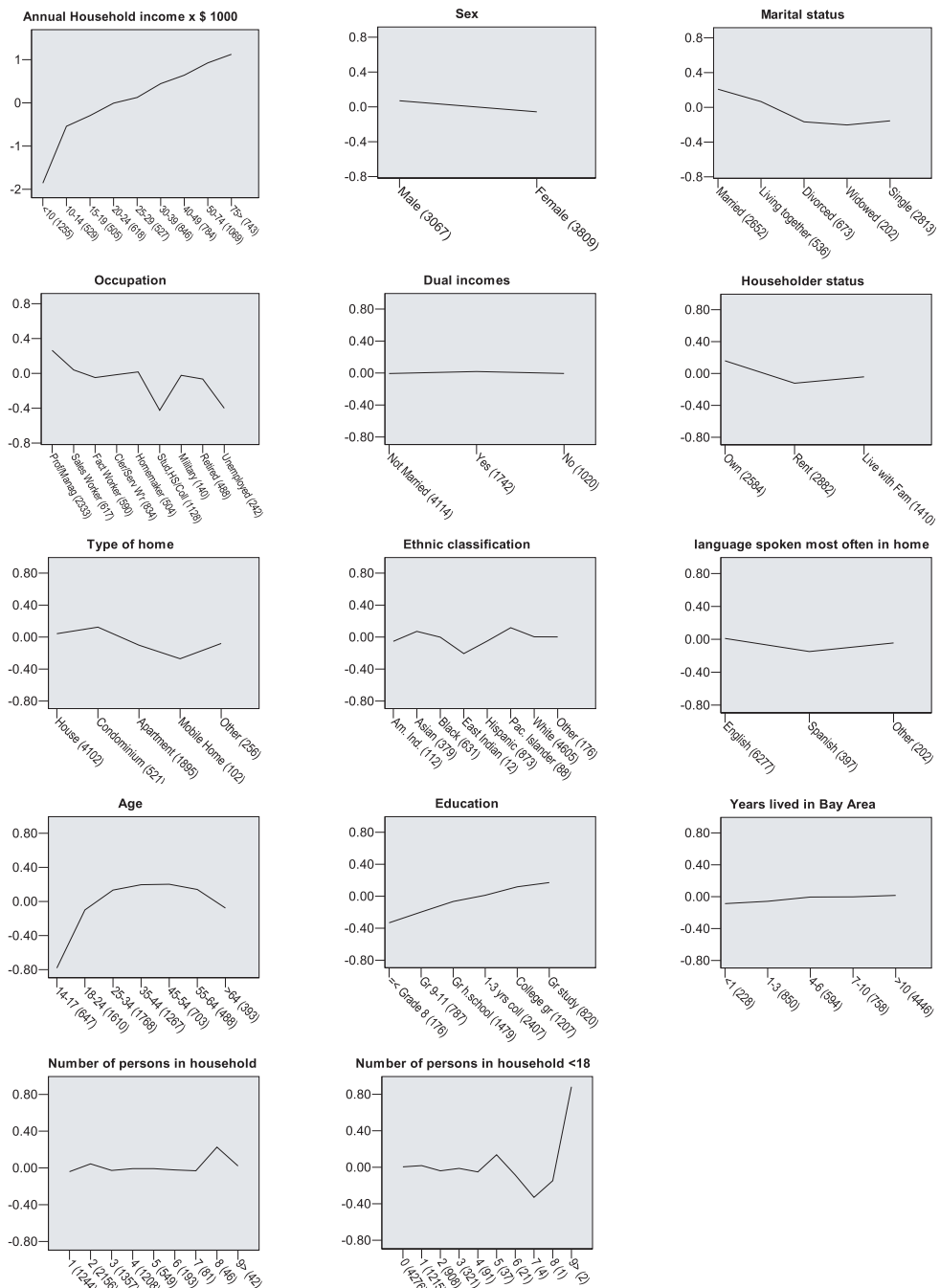
Figure 3.7. CATREG transformations for the demographic data (response ordinal, predictors nominal). The y-axis represent the quantifications multiplied with the regression coefficient for the predictor. The figures in brackets following the category labels are the category frequencies.
