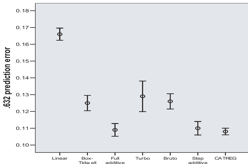
Figure 3.1. .632 Bootstrap estimates of prediction error. The bars around the estimates represent the estimated Monte Carlo standard error.
