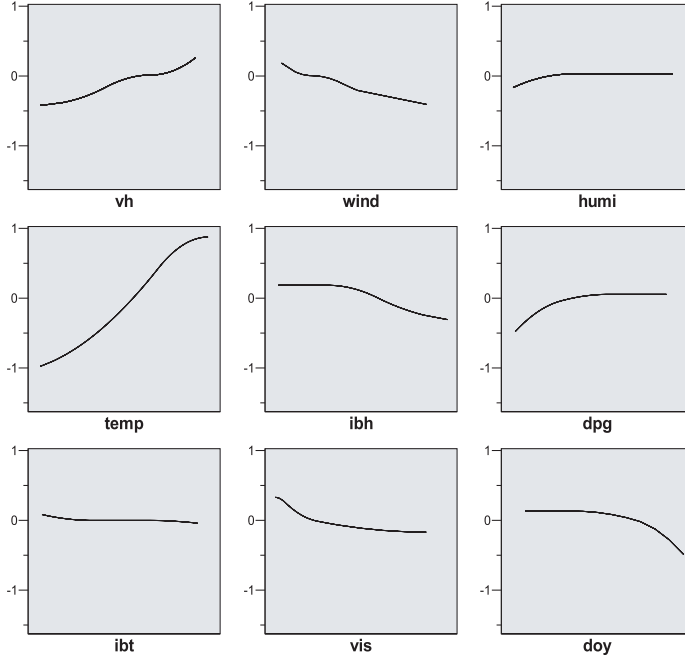
Figure 3.6. CATREG monotonic spline transformations for the recoded ozone data. The y-axis represent the quantifications multiplied with the regression coefficient for the predictor.
