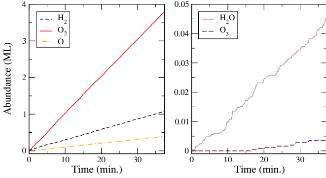
Fig. 4. Surface abundances of O, \text{O}_2 , \text{O}_3 , \text{H}_2 , and \text{H}_2\text{O} in time for the upper-limit simulation. One should realize that the total amount of deposited ice over the course of this simulation is 360 ML. The dominant component, by far, is \text{CO}_2 (not shown) because of its high flux.
