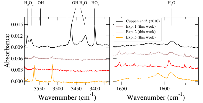
Fig. 2. RAIR difference spectra from a co-deposition of H and 16 O 2 from Cuppen et al. (2010), H 2 , CO 2 and 18 O (experiment 1), CO 2 and 18 O (experiment 2). Spectra are baseline corrected and offset for clarity. The spectra corresponding to experiments 1, 2 and 5 are scaled with a factor 3. Note that the multitude of peaks in the right panel for experiments 1 and 2 are due to water vapor in the setup, and the peaks at 3515 and 3564 cm -1 are also visible in a “pure” CO 2 spectrum.
