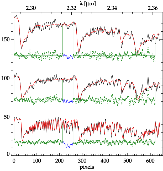
Fig. 3. Example of CO absorption line spectra (black) of a Voronoi bin of the full data cube (upper spectrum), a Voronoi bin of the cleaned data cube (middle spectrum) and of a single star (lower spectrum). The red lines are the ppxf -fits to the data. The blue regions are not fitted, as there is a strong telluric absorption line in this wavelength region. Green dots are the residuals of the fits. The fluxes of the spectra are scaled for this plot.
