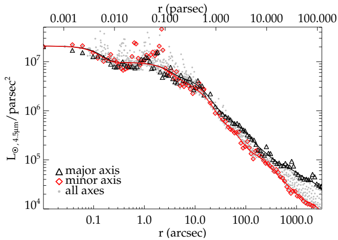
Fig. 15. Surface brightness profile derived from a dust and extinction corrected Spitzer /IRAC 4.5 \mu\text{m} image and NACO K -band mosaic for the central 30'' . Black triangles denote measurements along the major axis, and red diamonds along the minor axis, the grey data points are all measurements, at all axes. The spikes in the profile are due to individual bright stars. Solid lines illustrate the Multi-Gaussian Expansion (MGE) fit to the data.
