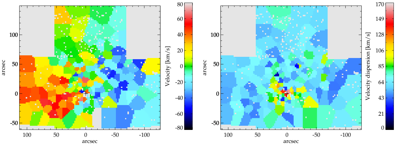
Fig. 5. Same as Fig. 4, but for the cleaned data cube. White pixels mark regions where there was no signal left after cutting out stars.
