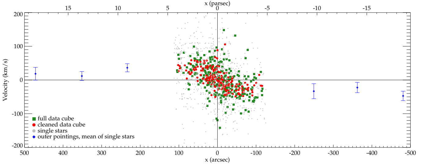
Fig. 10. Position-velocity diagram along the Galactic plane for the velocity maps of Figs. 4 and 5. Results from our full ISAAC data cube are shown as green rectangles, red circles show the result from the cleaned data cube, which contains only faint cluster member stars. Grey dots denote velocity measurements from single stars, the blue diamonds are the mean velocities of the bright stars at the outer fields, corrected for perspective rotation.
