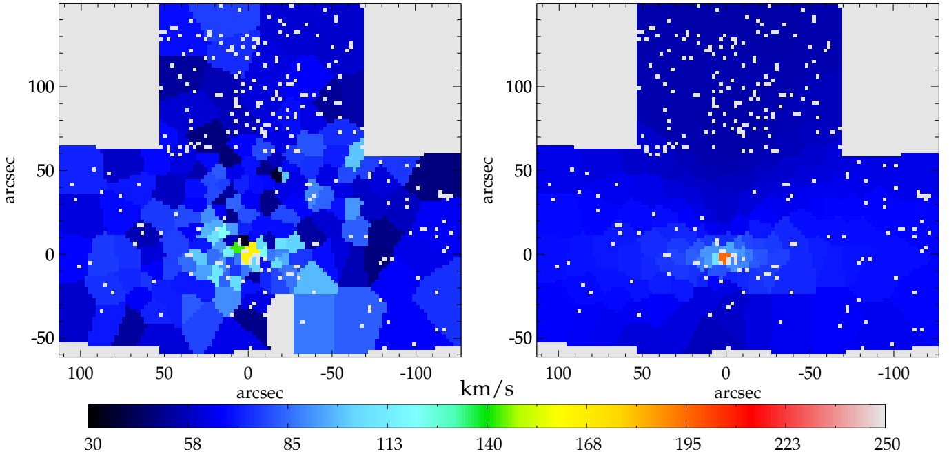
Fig. 16. Result of the two-dimensional Jeans model with anisotropy \beta_{\text{const}} = -0.3 , mass-to-light ratio M/L = 0.56 , and black hole mass M_{\bullet} = 1.7 \times 10^6 M_{\odot} . The left panel shows ISAAC data of the cleaned cube, for the root-mean-square velocity V_{\text{rms}} = \sqrt{V^2 + \sigma^2} , and the right panel is the best-fit model. The grey pixels mark regions, which contain no information. One bin was excluded from the fit due to its high uncertainty and low light-to-noise, and it is also shown in grey on the left panel .
