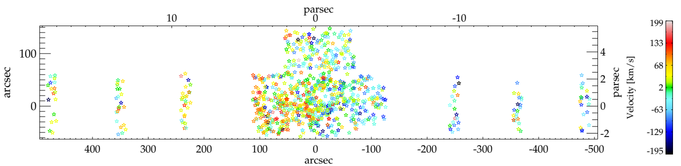
Fig. 6. Velocity map of 1094 bright stars ( K \leq 11.5^m ) with CO absorption lines in the colour interval 1.5^m \leq H - K \leq 3.5^m . We plot only stars with S/N > 12 and |v| < 200 \text{ km s}^{-1} .
