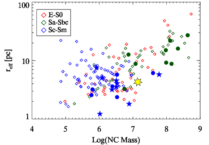
Fig. 18. Nuclear cluster mass M_{\text{NSC}} – effective radius r_{\text{eff}} relation for nuclear star clusters, based on Seth et al. (2008a) with data from Walcher et al. (2005) ; Rossa et al. (2006) shown as filled symbols and Böker et al. (2002) ; Carollo et al. (1997, 1998, 2002) ; Côté et al. (2006) as open symbols. The yellow star is the result for the Milky Way nuclear star cluster within an effective radius of 4.2 \text{ pc} ( Schödel et al. 2014 ).
