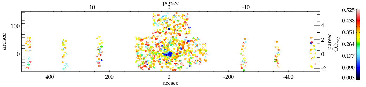
Fig. 14. CO index map of 1153 bright stars ( K \leq 11.5^m ) with S/N > 12 . Filled blue star symbols denote stars with \text{CO}_{\text{mag}} < 0.09 , which are younger than 300 Myr.
