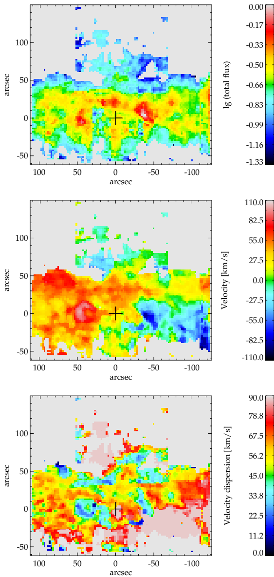
Fig. B.1. Results of the single Gaussian fit to the H 2 gas emission line. Upper panel: flux in logarithmic scaling and with respect to the maximum flux. Middle panel: velocity in \text{km s}^{-1} . Lower panel: velocity dispersion in \text{km s}^{-1} , corrected for the instrumental dispersion ( \sigma_{\text{instr}} \approx 27 \text{ km s}^{-1} ). The coordinates are centred on Sgr A* and along the Galactic plane with a position angle of 31^\circ 40' . The cross marks the position of Sgr A*.
