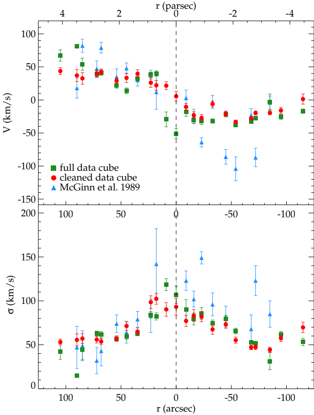
Fig. 13. Velocity ( upper panel ) and velocity dispersion profile ( lower panel ) along the major axis, with IRS 16 as the centre. We applied the binning of McGinn et al. 1989 (blue), extended by five additional binning apertures. Results from our full ISAAC data cube are shown as green rectangles, red circles show the result from the cleaned data cube, and blue triangles denote the data from McGinn et al. (1989).
