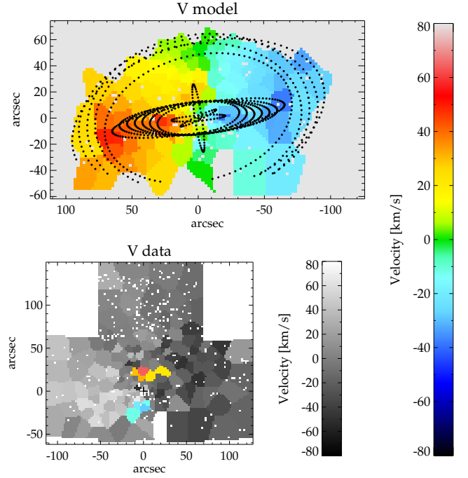
Fig. 8. Upper panel: kinematic model velocity map of the cleaned data cube. Black dots denote the best fitting ellipses. The model goes only to r \sim 100'' along the Galactic plane and to \sim 60'' perpendicular to it. The Voronoi bin with the highest uncertainty was excluded from the model. Lower panel: the velocity map as in Fig. 5 shown in grayscale, the bins that show rotation perpendicular to the Galactic plane are overplotted in colour scale.
