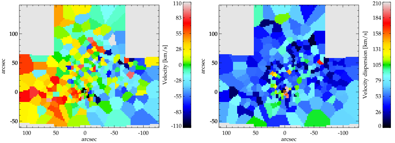
Fig. 4. CO absorption line map of velocity, and velocity dispersion (left, and right, respectively) obtained by using the full data cube. Both, velocity and velocity dispersion are in units of \text{km s}^{-1} . The coordinates are centred on Sgr A* and along the Galactic plane with a position angle of 31^{\circ}40' . The plus sign marks the position of Sgr A*. The velocity is in the local standard of rest, Galactic north is up, Galactic east is left.
