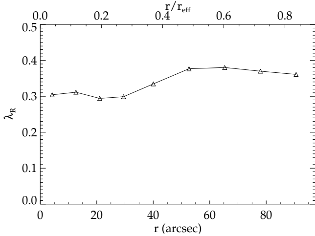
Fig. 9. Specific angular momentum \lambda_R profile calculated in ellipses with ellipticity \epsilon = 0.29 (Schödel et al. 2014), and plotted against the mean radius of the ellipses. The upper x -axis of the plot displays the ratio of r/r_{\text{eff}} , where r_{\text{eff}} is the effective radius ( r_{\text{eff}} = 4.2 pc, Schödel et al. 2014).
