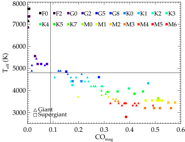
Fig. 7. Relationship between effective temperature T_{\text{eff}} in K and the CO index \text{CO}_{\text{mag}} for giant (triangle symbol) and supergiant (square symbol) stars of the IRTF Spectral Library (Rayner et al. 2009). Different colours denote a different spectral type. The black horizontal line marks 4800 K, the black vertical line marks \text{CO}_{\text{mag}} = 0.09 .
