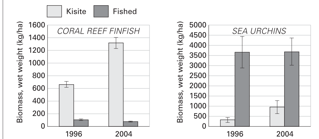
Figure 13.1 The biomass of coral reef finfish and sea urchins at Kisite and fished sites (Kanamai and Vipingo) in 1996 and 2004. (modified from McClanahan et al. 2006)
