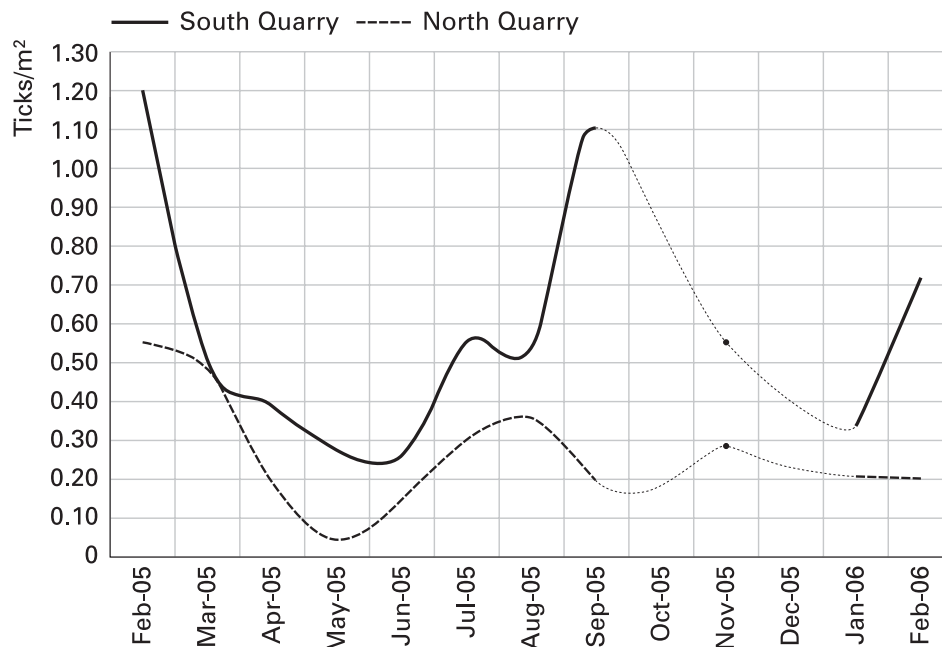
Figure 16.1 Tick densities (mean monthly number/m 2 ) pooled for sample sites in Bamburi North and Bamburi South quarries from Feb. 2005 to Feb. 2006. (No samples were taken in Oct. and Dec.)
