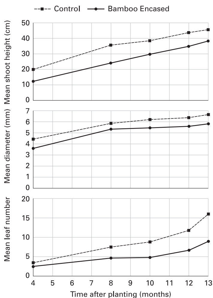
Figure 9.2 Growth performance of Rhizophora saplings at Gazi Bay
