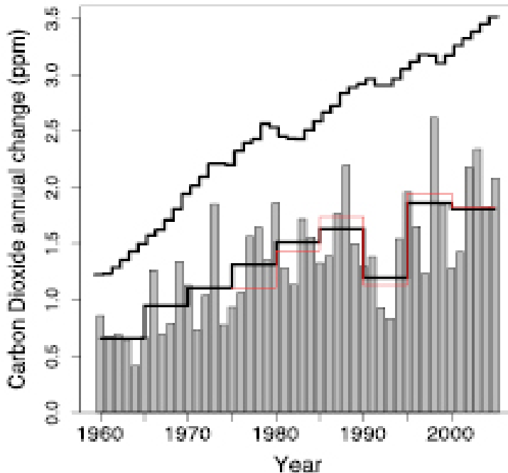
Figure 1.1 CO 2 emissions and increases 3
