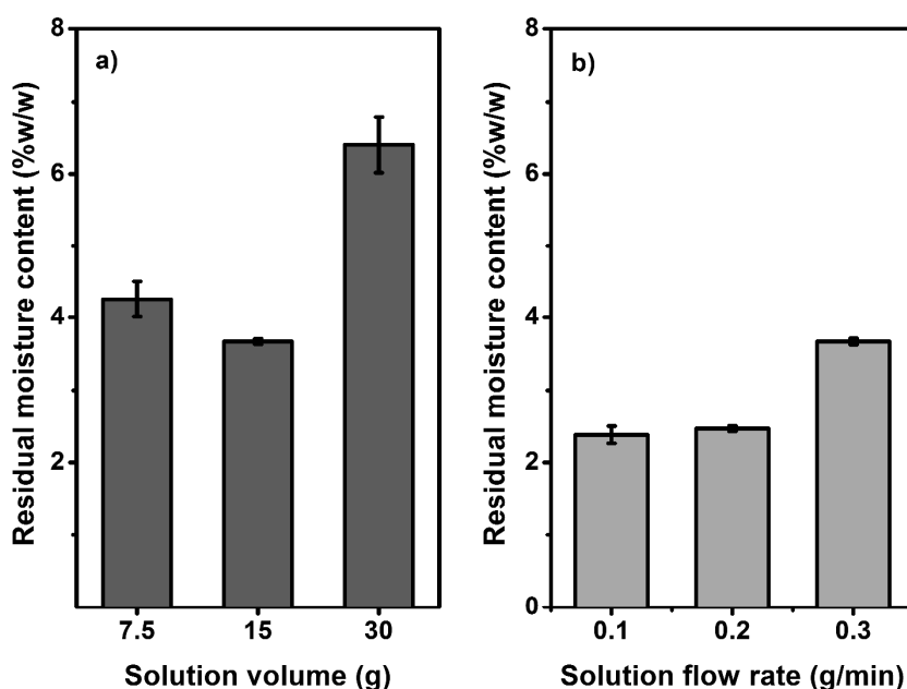
Fig. 1 Effect of a) feed solution volume (feed rate: 0.3 g/min) and b) feed rate (feed volume: 15 g) of an aqueous 5% (w/w) trehalose solution with 500 g/min CO 2 flow on the residual moisture content of the obtained powder, using the 4L drying chamber (conditions D, E, F and B, C, E; see Table 3).
