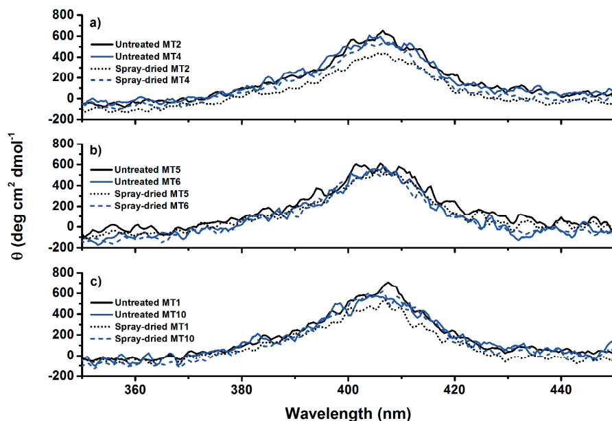
Fig. 2 Near/Vis-CD spectra at the Soret band (409 nm) of untreated myoglobin with trehalose and \text{scCO}_2 spray-dried myoglobin with trehalose, prepared in (a) phosphate buffer, (b) citrate and histidine, and (c) buffer-free solution. Spray-dried myoglobin formulations were conducted at 130 bar and 37 °C. MT2 and MT4 = myoglobin/trehalose in 10 and 150 mM phosphate buffer, MT5 = myoglobin/trehalose in 10 mM citrate, MT6 = myoglobin/trehalose in 25 mM histidine, MT1 and MT10 = 5 and 20 mg/ml myoglobin with 50 and 200 mg/ml, respectively, of trehalose in water. All untreated solutions were freshly prepared at pH 6.2. For formulation compositions, see Table 2.
