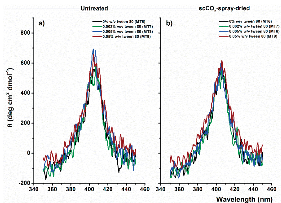
Fig. 3 Near/Vis-CD spectra at the Soret band (409 nm) of untreated formulations (a) and \text{scCO}_2 spray-dried myoglobin/trehalose formulations (b). Spray-dried myoglobin formulations (MT6-MT9 in 25 mM histidine, pH 6.2) contained 0-0.05% polysorbate 80 were prepared at 130 bar and 37 °C. For formulation compositions, see Table 2.
