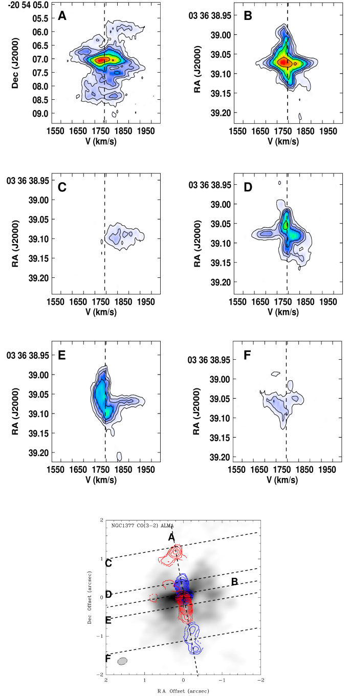
Fig. 3. Position-velocity (PV) diagrams showing gas velocities in six different slits: A ) along the jet axis; B ) perpendicular to the jet axis through the nucleus; C ) perpendicular to the jet axis at 1''.2 to the north; D ) perpendicular to the jet axis at 0''.25 to the north; E ) perpendicular to the jet axis at 0''.25 to the south; F ) perpendicular to the jet axis at 1''.2 to the south. Contour levels are 3.1 \times (1, 3, 5, 9, 18, 36)\text{ mJy beam}^{-1} thus the first level is at 4\sigma . The colour scale range from 2 to 156\text{ mJy beam}^{-1} .
