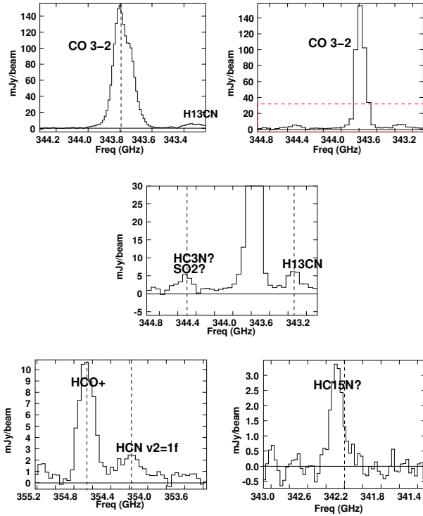
Fig. A.1. Spectra of the nuclear emission in NGC 1377. Dashed vertical line indicates v = 1740 \text{ km s}^{-1} . Top panels: CO 3–2 in high- ( left ) and low- ( right ) resolution spectral mode. The dashed red box of the right panel indicates the zoomed-in region in the next panel. Centre: zoomed-in spectrum showing detections of \text{H}^{13}\text{CN } J = 4-3 and either \text{HC}_3\text{N } J = 38-37 \nu_4 = 1, \nu_7 = 1 or \text{SO}_2 16(4,12)-16(3,13) . Bottom: panels showing detections of \text{HCO}^+ J = 4-3 , \text{HCN } J = 4-3 \nu_2 = 1f ( left ) and a line that we tentatively identify as \text{HC}^{15}\text{N } J = 4-3 . All spectra apart from in panels 2 and 3 have Gaussian smoothed with FWHM of two channels. In panels 2 and 3 there has been no smoothing but frequency resolution is reduced by a factor of 3 (these data stem from another spectral window than that presented in the first panel).
