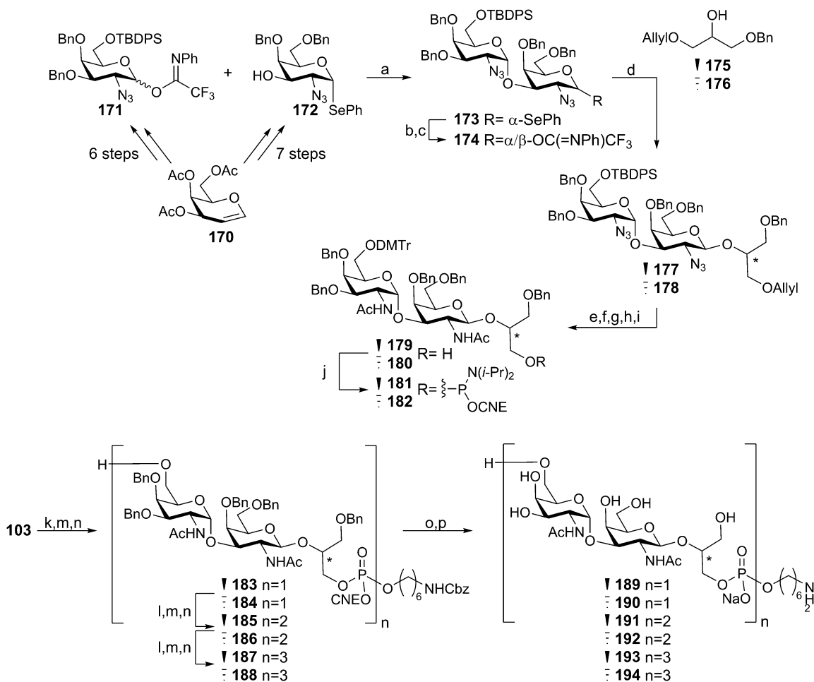
Scheme 15 Enterococcus faecium WTA synthesis. Reagents and conditions: (a) TfOH, DCM, 0^\circ\text{C} , 58%; (b) NIS, THF/ \text{H}_2\text{O} ; (c) \text{CF}_3\text{(=NPh)Cl} , \text{K}_2\text{CO}_3 , acetone, quant over 2 steps; (d) 175 or 176 , TfOH, MeCN/EtCN/DCM, -40^\circ\text{C} , 177 : 90% 178 : 80%; (e) \text{PMe}_3 , dioxane/ \text{H}_2\text{O} ; (f) \text{Ac}_2\text{O} , \text{NEt}_3 , DCM; (g) TBAF, THF; (h) DMTrCl, \text{NEt}_3 , DCM; (i) (1) Ir(COD)(Ph 2 MeP) 2 , THF; (2) \text{NaHCO}_3 , \text{I}_2 , \text{H}_2\text{O} /THF, 179 : 28% over 5 steps, 180 : 46% over 5 steps; (j) di-isopropylethylamine, N,N -di-isopropylamino-2-cyanoethyl-chlorophosphite, DCM, 181 : 85% 182 : 62%; (k) DCI, 179 or 180 , MeCN; (l) DCI, 181 or 182 , MeCN; (m) CSO, MeCN; (n) 3% TCA, DCM, 183 : 72%, 184 : 80%, 185 : 62%, 186 : 64%, 187 : 69%, 188 : 67%; (o) \text{NH}_3 (conc), dioxane; (p) Pd(0), \text{H}_2 , AcOH, \text{H}_2\text{O} , 189 : 73%, 190 : 57%, 191 : 44%, 192 : 45%, 193 : 49%, 194 : 56%.
