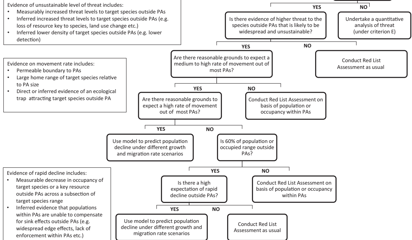
Fig. 4. Decision tree for threat assessment of protection-reliant species.
