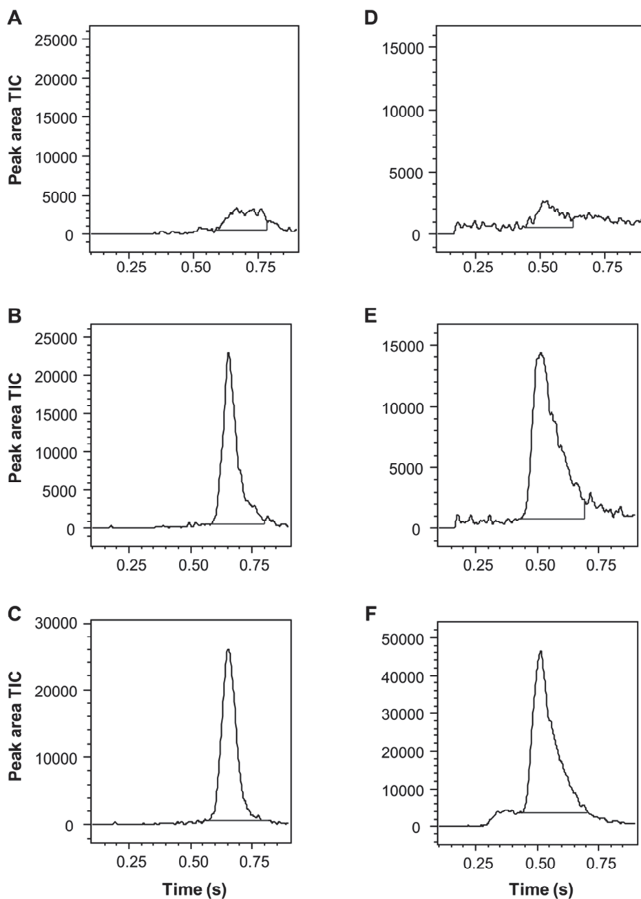
Figure 2. Typical chromatograms of A) nonspecific binding of DCPX (31 pM), B) total binding of DCPX (242 pM), and C) [ ^2 H]DCPX (2 nM) in eluate containing hA 1 AR membrane matrix, and of D) nonspecific binding of ZM-241,385 (42 pM), E) total binding of ZM-241,385 (289 pM), and F) [ ^2 H]ZM-241,385 (2 nM) in eluate containing hA 2A AR membrane matrix. The straight lines below the peaks delineate area of peak integration.
