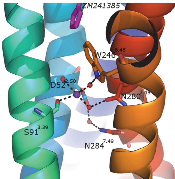
Figure 1. Residues in or close to the sodium ion binding site that we subjected to an alanine scan in the hA 2A AR, mapped on the crystal structure of the hA 2A AR in the inactive ZM-241,385 and sodium ion bound conformation (PDB 4E1Y) 4 . Residues Asp52 2.50 , Ser91 3.39 , Trp246 6.48 , Asn280 7.45 , and Asn284 7.49 (represented by sticks, of which red and blue sticks are oxygen and nitrogen atoms, respectively) coordinate the sodium ion (purple sphere). Numbering of the residues follows the Ballesteros-Weinstein system for comparison of positions between GPCRs. 7 Water molecules interacting with the sodium ion are represented by red spheres; hydrogen bonds are represented by black dotted lines; receptor backbone is represented by ribbons. Purple stick structure on top represents (part of) co-crystallized ZM-241,385.
