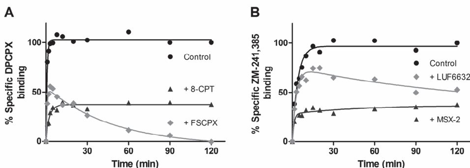
Figure 6. Competition association of DPCPX on hA_1AR in the presence or absence of 250 nM 8-CPT and 250 nM FSCPX (A), and of ZM-241,385 on hA_{2A}AR in the presence or absence of 90 nM MSX-2 and 15 nM LUF6632 (B). Graphs show mean values of one representative MS binding competition association experiment performed in duplicate.
