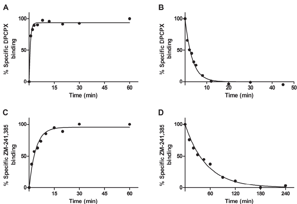
Figure 5. Association (A, C) and dissociation (B, D) of DPCPX on hA_1AR (A, B) and ZM-241,385 on hA_{2A}AR (C, D). Graphs show mean values of one representative MS binding association or dissociation experiment performed in duplicate.
