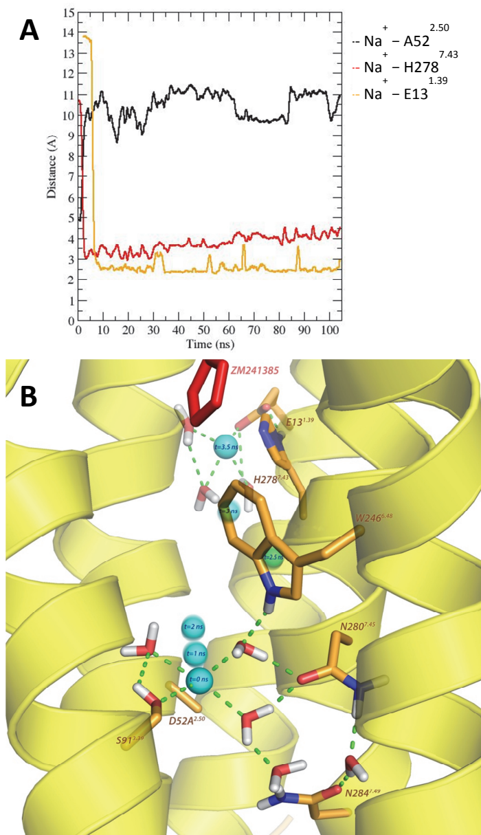
Figure 5. A) Average distance in Å of sodium ion from Glu13 1.39 (Oε), Ala52 2.50 (Cα), and His278 7.43 (Nδ) as a function of the simulation time for the D52A 2.50 mutant. Graphs represent means from three independent simulations. B) 3D representation of the migration pathway of the sodium ion (cyan sphere, with labels indicating the occupancy at averaged MD simulation windows) from its putative binding site towards the vestibular pocket formed by Glu13 1.39 and His278 7.43 . The residues and water molecules interacting with the sodium ion are represented in sticks, and hydrogen bonds represented by green dotted lines.
