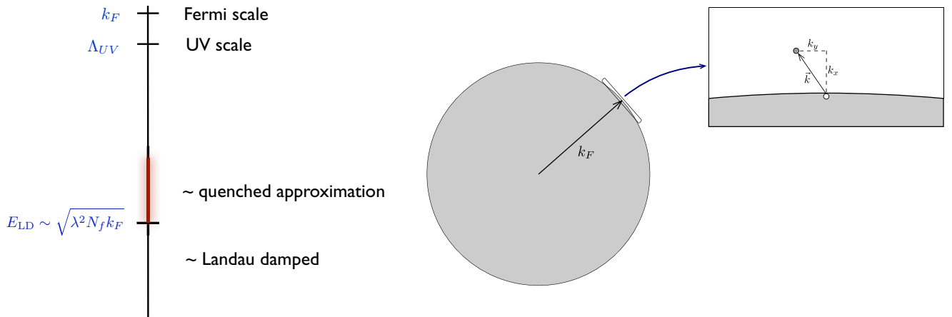
FIG. 3. (Left) The energy scales relevant to 2+1 dimensional finite density fermions coupled to a massless boson. We assume the theory is already truncated at a UV cutoff \Lambda_{UV} lower than the Fermi scale k_F . The quenched N_f \rightarrow 0 limit focuses in on the intermediate energy regime right above the scale E_{LD} \sim \sqrt{\lambda^2 N_f k_F} where Landau damping becomes important. (Right) A small patch of the Fermi surface. In a small region near the Fermi level, the surface curvature is negligible. Fermionic excitations can acquire both orthogonal k_x and tangent k_y momenta, but the latter does not contribute to the kinetic energy of the excitation. In the N_f \rightarrow 0 limit, each patch decouples from other parts of the Fermi surface.
