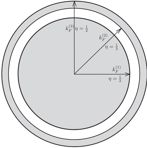
FIG. 4. The emergent Fermi surface structure at low energy in the 2+1-dimensional quenched planar patch quantum critical metal. Due to the interactions, the naive single Fermi surface is topologically unstable. The excitations around the Fermi surfaces are not well-defined quasiparticles, instead they have a continuous spectrum corresponding to a Green's function of the type G(\omega, k) \sim (\omega - vk)^{-\eta} with scaling dimensions \eta . The different values of \eta at each of the emergent singular surfaces are mentioned.
