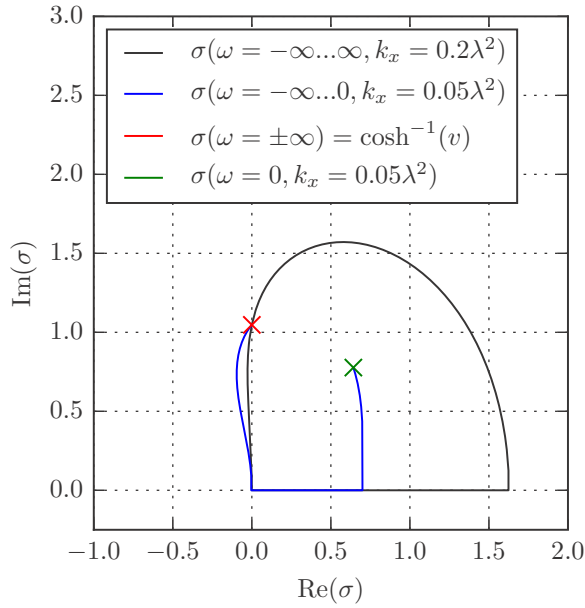
FIG. 10. This figure shows a closed contour of integration for the sum rule and an open contour for calculating the occupation number integral, v = 0.5 .
