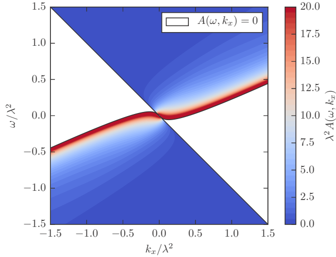
FIG. 5. Fermionic spectral function for v = 0.5 . It is identically zero in the white region.
