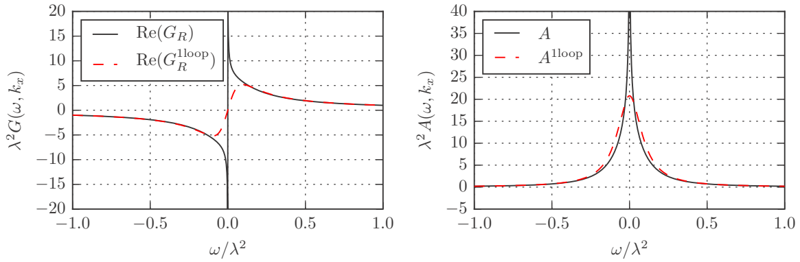
FIG. 7. The real and the imaginary parts of the Green's function at the middle Fermi surface ( k_x = 0, v = 0.5 ) as a function of \omega (solid line), compared with the corresponding one-loop result (dashed).
