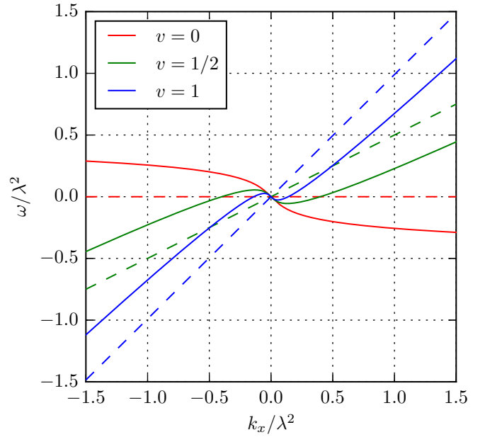
FIG. 6. The dispersion relation (the zeros of G^{-1} ) for different v in the interacting theory (solid line) and the free theory (dashed).
