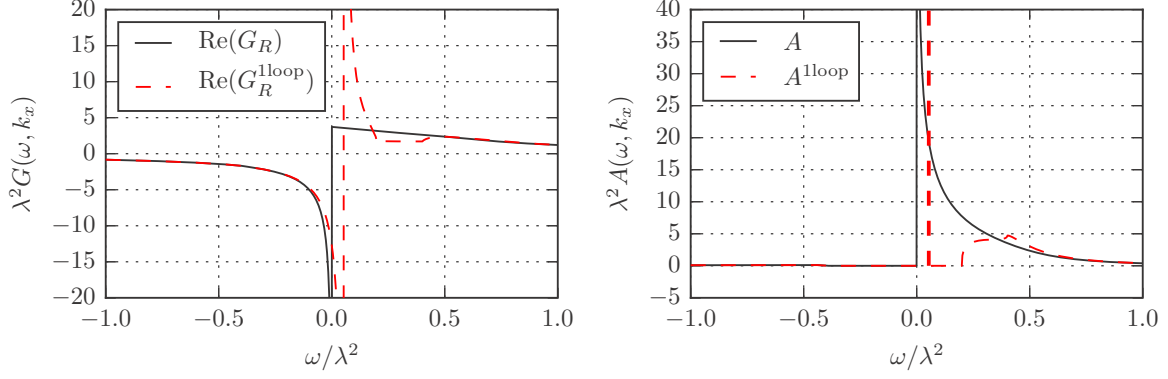
FIG. 8. The real and the imaginary part Green's function at the outer Fermi surface ( k_x = k_x^* \approx 0.4\lambda^2 and v = 0.5 ) as a function of \omega (solid line), and the one-loop truncated result (dashed). The spectral weight of the one-loop approximation is concentrated to a \delta function, whereas the spectral weight of the full result is spread in the power-law singularity.
