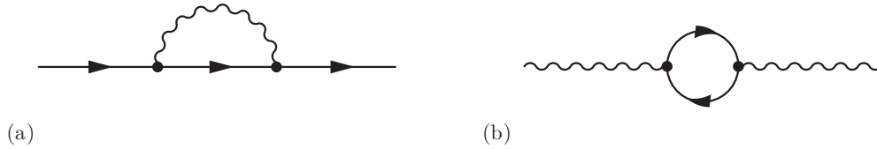
FIG. 1. One-loop corrections to fermion (a) and boson (b) self-energies due to Yukawa interaction. For a gapless boson, (b) is the one-loop contribution to Landau damping: this contribution to the self-energy can dominate in the IR. This term (b) is clearly proportional to the number of fermions N_f in contrast to the one-loop correction to the fermion self-energy (a). In the limit N_f \gg N_b , the boson self-energy/Landau damping therefore dominates, whereas it is suppressed in the opposite limit N_f \ll N_b .
