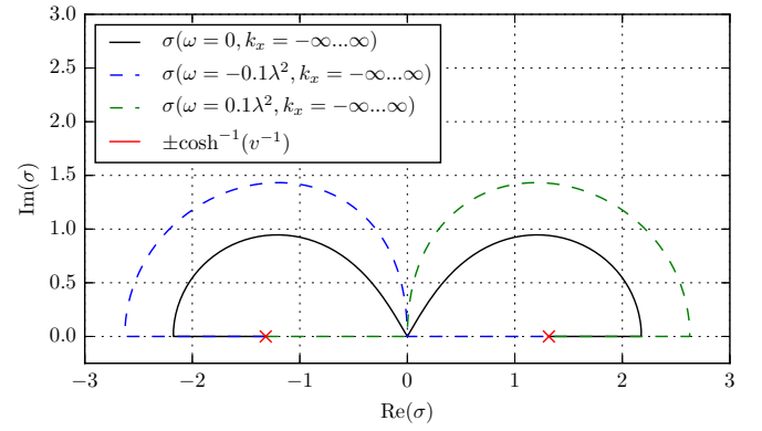
FIG. 11. Integration contours for calculating density of states. The integrand and locations of the endpoints are independent of \omega but since the integrand has poles at the endpoints the direction of approach matters. The poles are always approached along the real axis and this figure shows the three possible configurations, v = 0.5 .
