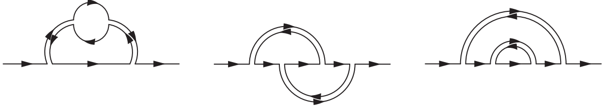
FIG. 2. The two-loop contributions to the fermion self-energy in theory in Eq. (3). The quenched limit where N_f \rightarrow 0 only suppresses the fermion loop contribution (a), whereas matrix large N limits, where the boson is a N \times N matrix \phi_i^j and the fermion a N -component vector \psi_i also suppress crossed diagrams of type (b). This is evident in double line notation of the same Feynman diagrams where the fermion is written as a single line (it has one index) and the matrix-valued boson as two lines (it has two indices). Indices have to match at interactions; each closed loop therefore corresponds to a sum over this index and gives a weight N to the diagram. We then see that the crossed diagram has no loops and is thus subdominant in N to other diagrams at the same order in the coupling constant.
