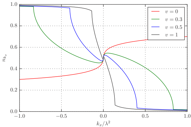
FIG. 9. The occupation number for different v as a function of momentum. We can see the effect of the multiple sharp fermi surfaces, the non-Fermi-liquid behavior is also apparent as a nonmonotonic behavior of the occupation number.
