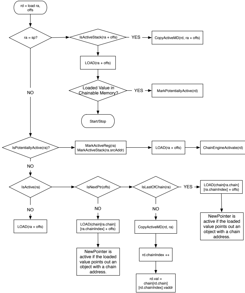
Figure 5.5: Active Pointer Tracking
