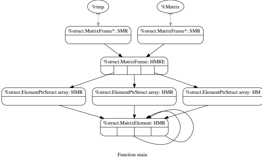
Figure 2.3: DSGraph for main function of SPMATVEC benchmark.
