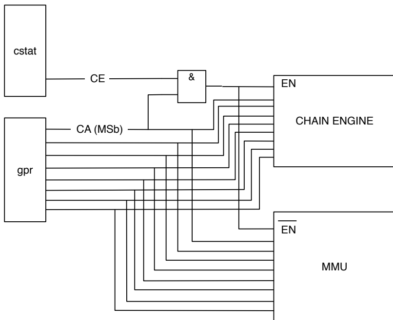
Figure 5.1: Logic for detecting chainable addresses using a dedicated bit. In order to allow the enabling of chaining support per application, a dedicated chain status register (cstat) has a special bit that allow the enabling / disabling of the chaining engine. If this bit is set and the chain address bit is set in the address located in one of the GPRs, the the address is routed to the chain engine instead of the MMU.
