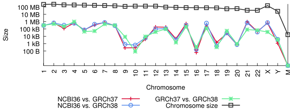
Figure 3.3: HGVS Description lengths of the extraction algorithm per chromosome.
