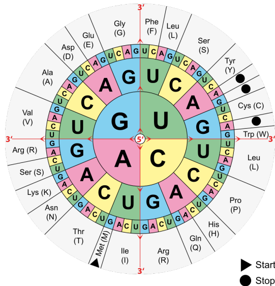
Figure 2.2: A schematic representation of the genetic code where the RNA notation is used. Image by Mouagip [Public domain], via Wikimedia Commons.
