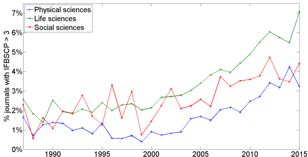
Fig 3. Percentage of journals with IFBSCP > 3 (different fields of science).
