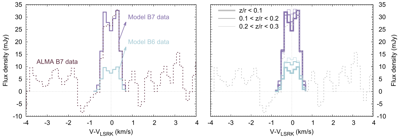
Figure 2. Left: line profile extracted from the stacked observed B7 \text{CH}_3\text{OH} channel map within the 3\sigma contour of the 317 GHz continuum (dark red dashed lines) compared with the stacked B6 and B7 model line profiles from the best “by-eye” model fit for z/r < 0.1 (light blue and purple lines, respectively). Right: best “by-eye” fits for models in which methanol is present in different layers: z/r \leq 0.1 , 0.1 \leq z/r \leq 0.2 , and 0.2 \leq z/r \leq 0.3 . In all models, methanol is located between 30 and 100 au.
