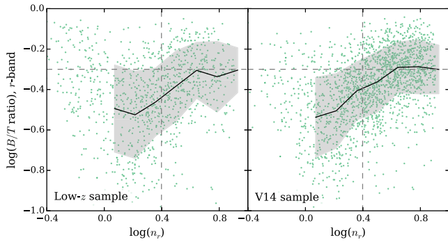
Figure 7. The relationship between n_r(\text{galaxy}) and B/T for two-component galaxies in the low- z sample (left-hand panel) and the V14 sample (right-hand panel). Overplotted as grey dashed lines are the low-/high- n cut at n_r = 2.5 , and the division between disc-/bulge-dominated galaxies at B/T = 0.5 . Solid black lines show the median fitted values whilst the shaded areas show the 1\sigma dispersion. We see a positive correlation between B/T and Sérsic index, implying that we can generally think of high- n galaxies as being bulge-dominated, and vice versa.
