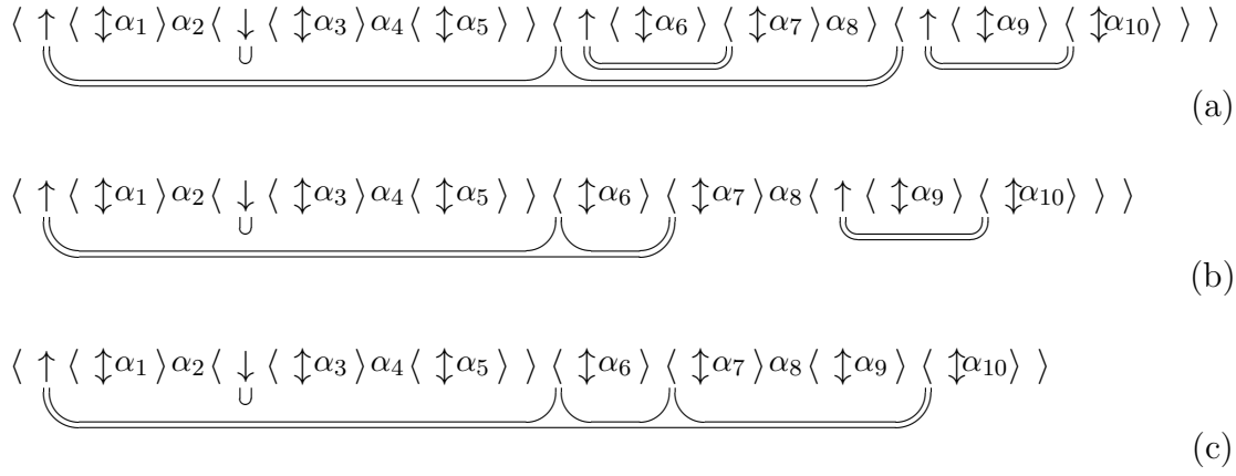
Figure 7.18: Fourth feature of the datastructure used in the implementation of the algorithm for minimality. Each occurrence of \uparrow or \downarrow has a circular, doubly-linked list of its consecutive expression-arguments. (a) The lists for an example DNA expression. (b) The result after substituting the \uparrow -subexpression \langle \uparrow \langle \downarrow \alpha_6 \rangle \langle \downarrow \alpha_7 \rangle \alpha_8 \rangle by its arguments. (c) The result after substituting the \uparrow -subexpression \langle \uparrow \langle \downarrow \alpha_9 \rangle \langle \downarrow \alpha_{10} \rangle \rangle by its arguments.
