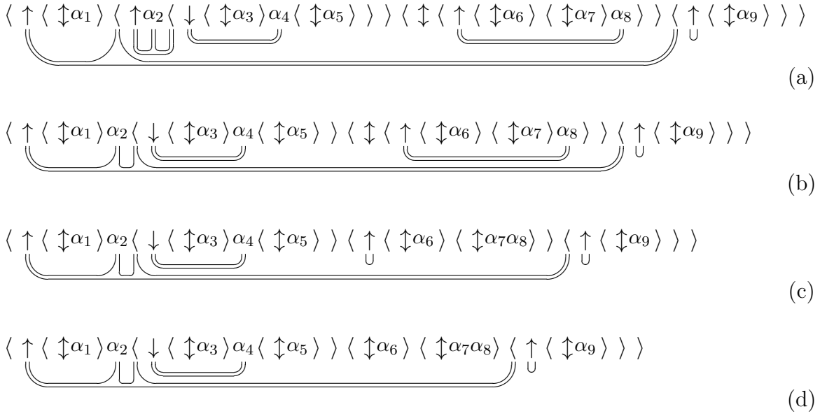
Figure 7.17: Third feature of the datastructure used in the implementation of the algorithm for minimality. Each occurrence of \uparrow or \downarrow has a circular, doubly-linked list of its non- \downarrow -arguments. (a) The lists for an example DNA expression. Note that the list is empty for the last occurrence of \uparrow . (b) The result after substituting the \uparrow -subexpression \langle \uparrow \alpha_2 \langle \downarrow \langle \downarrow \alpha_3 \rangle \alpha_4 \langle \downarrow \alpha_5 \rangle \rangle \rangle by its arguments. (c) The result after using procedure Make \uparrow ExprMinimal to substitute the \downarrow -argument \langle \downarrow \langle \uparrow \langle \downarrow \alpha_6 \rangle \langle \downarrow \alpha_7 \rangle \alpha_8 \rangle \rangle by \langle \uparrow \langle \downarrow \alpha_6 \rangle \langle \downarrow \alpha_7 \alpha_8 \rangle \rangle . As explained in the text, we do not need to insert the resulting \uparrow -argument into the list of non- \downarrow -arguments of the outermost operator \uparrow . (d) The result after substituting the \uparrow -subexpression \langle \uparrow \langle \downarrow \alpha_6 \rangle \langle \downarrow \alpha_7 \alpha_8 \rangle \rangle by its arguments.
