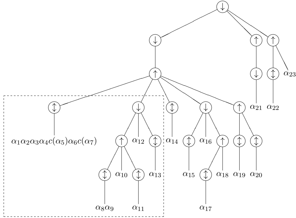
Figure 7.9: Structure tree of the example DNA expression for the algorithm for minimality, after five substitutions, (7.18). The dashed box encloses the part of the tree that has changed as compared to Figure 7.8.
