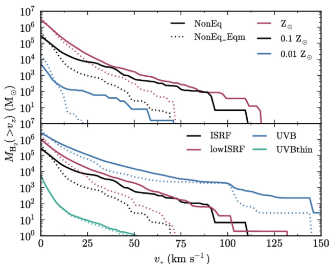
Figure 7. Mass of molecular hydrogen in particles moving away from the mid-plane of the disc with a vertical velocity >v_z , plotted as a function of v_z , for different metallicities (top panel) and for different radiation fields (bottom panel; see Table 1). We calculate the H_2 masses from simulations run using the full chemical model using non-equilibrium abundances (solid curves) and from the same simulations but with abundances set to chemical equilibrium in post-processing (dotted curves). We average these curves over 10 snapshots for each simulation, at intervals of 100 Myr. The mass of H_2 in outflowing gas ( >50 \text{ km s}^{-1} ) is generally much higher in non-equilibrium, e.g. by a factor of \sim 20 in the ISRF run.
