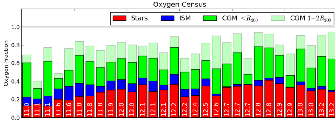
Figure 9. The oxygen budget for zoom haloes ordered by halo mass ( \log[M_{200}/M_{\odot}] ) indicated by rotated white numbers), where the amount of oxygen produced and released by all galaxies within R_{200} is normalized to one. The relative oxygen content in stars (red), the ISM (blue), and the CGM (within R_{200} , bright green; at 1-2R_{200} , faded green) is then summed relative to the total oxygen production, as in P14. For L^* and group haloes, there exists more oxygen in the CGM within 2R_{200} than in the galaxy (stars+ISM) itself. Up to half the oxygen generated by an L^* galaxy can be ejected beyond R_{200} . One difference with P14 is that we sum the stellar and ISM oxygen content for all (central and satellite) galaxies in the halo, where P14 only include the central galaxy for these quantities.
