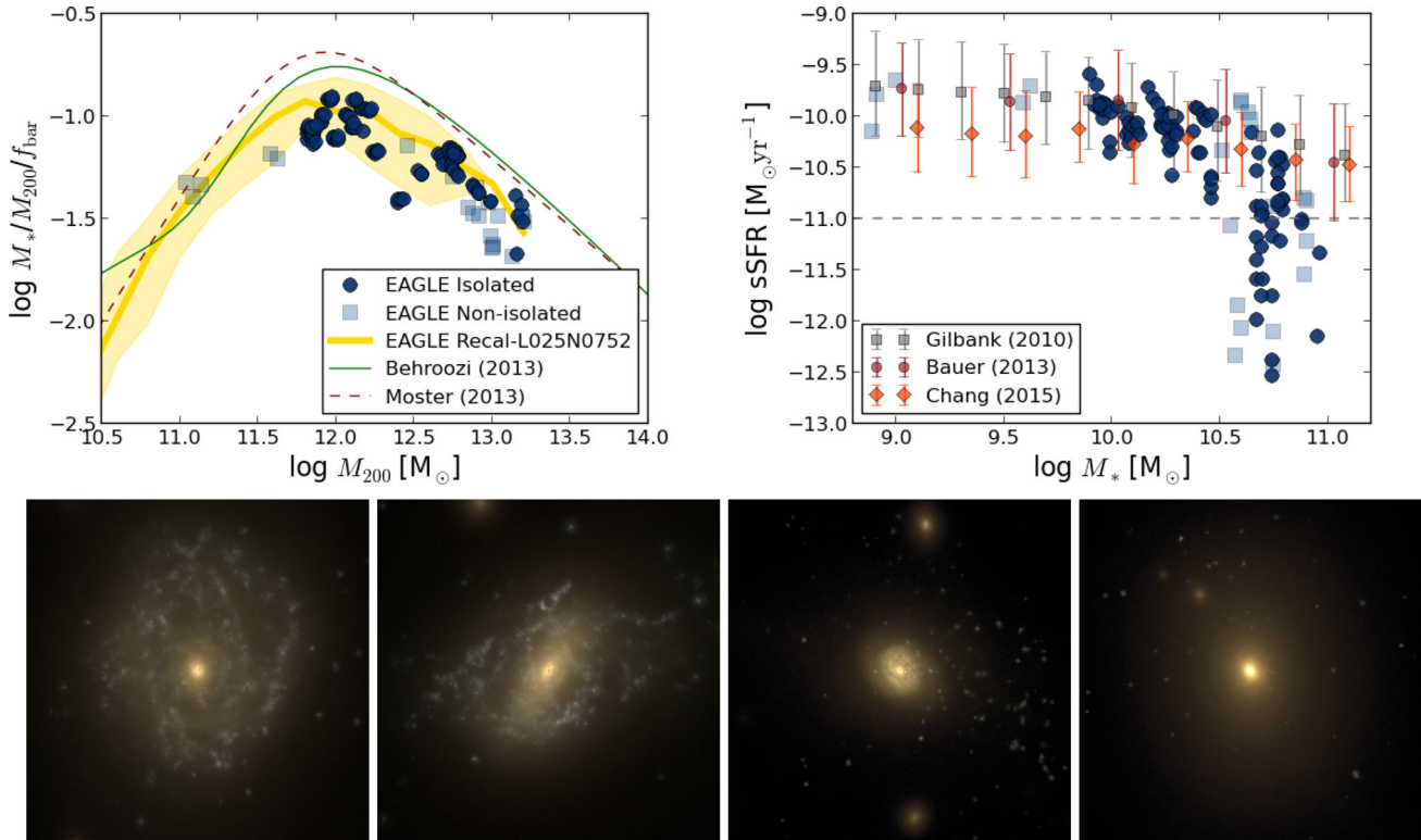
Figure 1. Stellar mass to halo mass ratio plotted as a function of halo mass of zoomed centrals (top left) and sSFR as a function of stellar mass (top right) from six redshifts ( z = 0.25 \rightarrow 0 ) that we use in our analysis. Galaxies that can be considered ‘isolated’ by COS-Halos criteria are indicated by dark circles, while transparent squares indicate galaxies with a neighbouring galaxy with M_* > 10^{10.3} M_\odot within 300 kpc. Three sub- L^* galaxies at z = 0.205 are also plotted as light circles. The thick yellow line is the fit to all centrals in the RECAL-L025N0752 simulation (S15) with the shading indicating the 1\sigma dispersion. Abundance matching results from Behroozi et al. (2013, solid green) and Moster et al. (2013, dashed red) at z = 0.2 are displayed on the left, and observations of the sSFR of star-forming galaxies as a function of M_* from Gilbank et al. (2010, grey squares), Bauer et al. (2013, brown circles), and Chang et al. (2015, orange diamonds) are displayed on the right. Bottom panels show simulated 50 kpc SDSS u -, g -, and r -band composite images, including dust, of two star-forming L^* galaxies and two group centrals – a recent merger and a passive galaxy (from left to right). All plots use M5.3 zooms.
