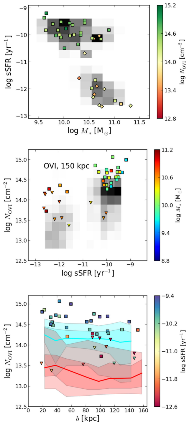
Figure 8. Probability distributions of mock observations from 100 SMOHALOS realization displayed in grey shading on a linear scale on the M_* -sSFR plane (top panel) and the N_{\text{OVI}} -sSFR plane (centre panel). COS-Halos data are plotted as in Fig. 7, but without error bars. The bottom panel shows median N_{\text{OVI}} as a function of impact parameter for the star-forming (cyan) and passive (red) SMOHALOS samples, including darker and lighter shading for 1\sigma and 2\sigma dispersions. There is hardly any overlap of the 1\sigma dispersions between the star-forming and passive samples.
