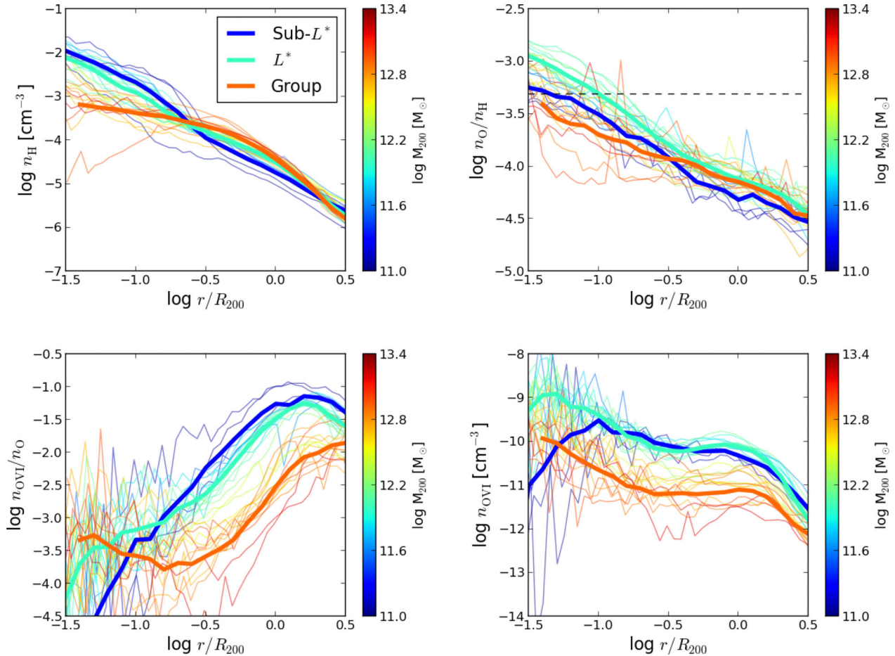
Figure 5. Radial profiles averaged in spherical shells of the hydrogen density ( n_{\text{H}} ), oxygen abundance ( n_{\text{O}}/n_{\text{H}} ), O VI ion fraction ( x_{\text{OVI}} \equiv n_{\text{OVI}}/n_{\text{O}} ), and O VI density ( n_{\text{OVI}} ) as a function of fractional virial radius from top left to bottom right at z = 0.205 . Individual haloes are shown as thin lines, and thick solid lines represent averages of sub- L^* , L^* , and group-sized haloes (blue, aquamarine, and orange). The dashed line in the top right-hand panel indicates the solar oxygen abundance ( n_{\text{O}}/n_{\text{H}} = 10^{-3.31} ). Lower mass haloes have higher densities in their centres (top left), and L^* mass haloes have the highest oxygen abundances in their centres (top right). x_{\text{OVI}} (bottom left) shows a strong trend with halo mass. Sub- L^* haloes ( <10^{11.5} M_{\odot} ) have the highest x_{\text{OVI}} owing to higher photoionized fractions, but this photoionized phase is greatly reduced in L^* haloes owing to higher pressures. Instead, L^* haloes are dominated by collisionally ionized O VI, and ion fractions only reach \sim 5 per cent at radii just beyond R_{200} . Group haloes have even lower x_{\text{OVI}} because the vast majority of the gas is too hot for O VI, and only gas beyond R_{200} approaches x_{\text{OVI}} of several per cent. The bottom right-hand panel, showing O VI densities, is the product of the previous three panels, and shows the higher O VI densities for sub- L^* and L^* haloes than for group haloes.
