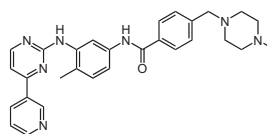
Imatinib
