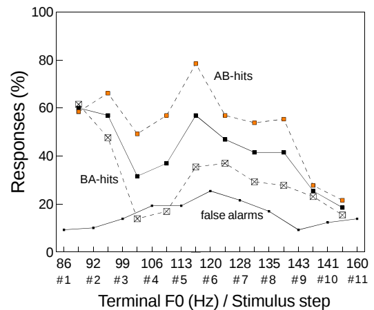
Figure 4. Percent hits (AB and BA-orders presented separately as well as averaged) and false alarms as a function of stimulus step number. (terminal F_0 of boundary tone).
