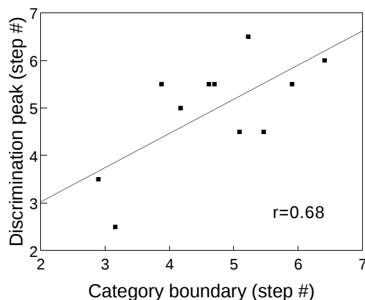
Figure 5. Location of peak in the individual discrimination function (averaged over AB and BA orders) against location of individual cross-over in identification task
