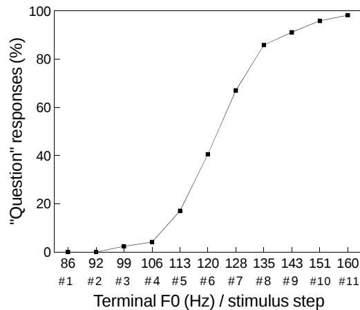
Figure 2. Percent 'question' responses as a function of stimulus step number. Data have been accumulated across all listeners.
