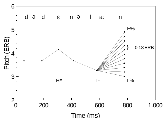
Figure 2. F_0 continuum (11 steps) between L-L% and L-H%.
