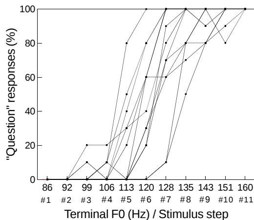
Figure 3. Percent 'question' responses as a function of stimulus step number. Data are presented for individual listeners.
