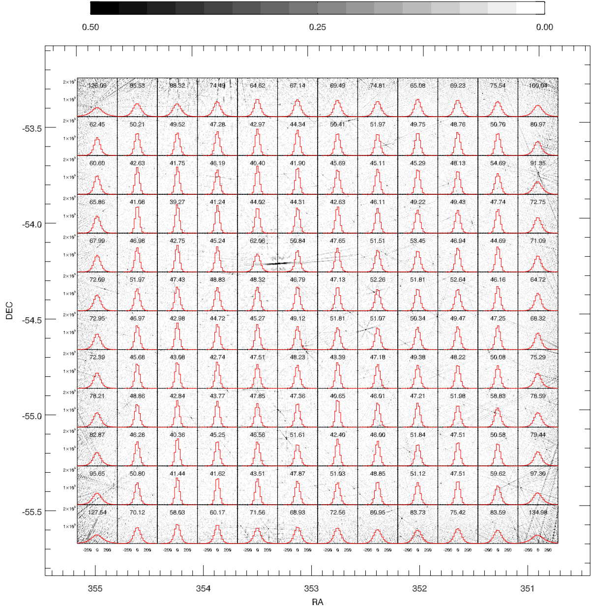
Fig. 1. Inverted greyscale of our XXL-S Pilot Survey mosaic at 2.1 GHz. The greyscale colourbar in units of mJy/beam is shown at the top. Overlaid are histograms of pixel flux distributions for different regions of the mosaic. The standard deviation for each region is indicated in each panel (in units of \mu\text{Jy/beam} ). The x -axis of the histograms shows flux density in \mu\text{Jy/beam} and the y -axis shows counts. The outer 500 pixels of the map have been excluded here since they are not considered in the source-finding process.
