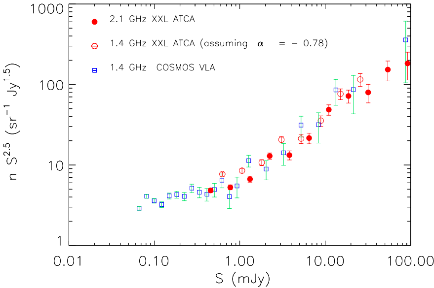
Fig. 6. Normalised differential source counts for the 2.1 GHz ATCA XXL-S survey (red filled dots), estimated 1.4 GHz ATCA XXL-S counts (assuming a spectral index of \alpha = -0.78 ; red open dots) and for the COSMOS VLA 1.4 GHz survey (blue open squares).
