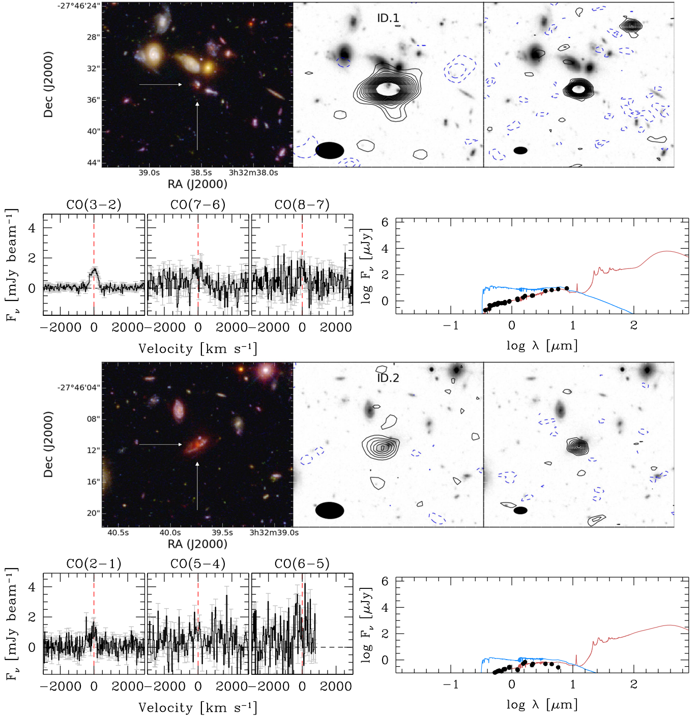
Figure 11. Top left: HST F105W/F775W/F435W RGB image of ID.1 and 2. The postage stamp is 20'' \times 20'' . Top center: HST F125W image of the same field. The map of the lowest- J accessible CO transition (in this case, CO[3–2]) is shown as contours ( \pm 2, 3, \dots, 20\text{-}\sigma [ \sigma(\text{ID.1}) = 0.78 \text{ mJy beam}^{-1} ; \sigma(\text{ID.2}) = 1.36 \text{ mJy beam}^{-1} ]; solid black lines for the positive isophotes, dashed blue lines for the negative). The synthesized beam is shown as a black ellipse. Top right: same as in the center, showing the 1.2 mm dust continuum. Bottom left: spectra of the CO lines encompassed in our spectral scan. Bottom right: spectral energy distribution. The red line shows the best MAGPHYS fit of the available photometry (black points), while the blue line shows the corresponding model for the unobscured stellar component. The main output parameters are quoted.
