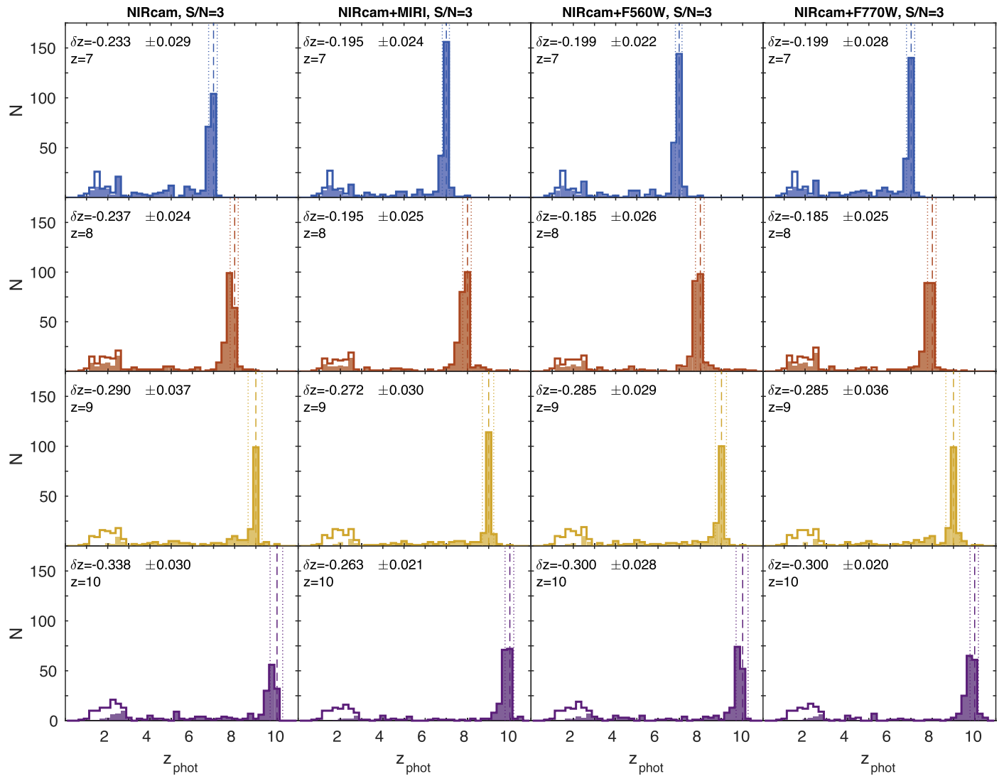
Figure 20. Same as Figure 17, but for S/N = 3 . The shaded area within each histogram corresponds to objects with more than four detections in total in the NIRCcam and MIRI bands, while open areas correspond to sources with less than four band detections.
