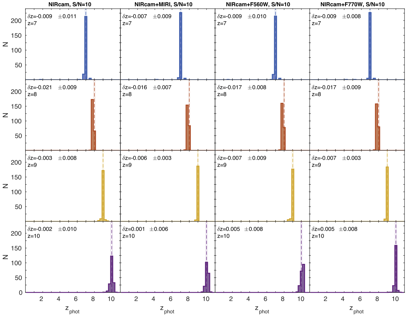
Figure 12. Photometric redshifts obtained for the BC03 simulated galaxies with (F150W) S/N = 10 at different fixed redshifts. From top to bottom: redshifts z = 7-10 . Photometric redshifts in each column are obtained with different combinations of bands. From left to right: eight NIRCam broadbands; eight NIRCam broadbands, MIRI F560W, and MIRI F770W; eight NIRCam broadbands and MIRI F560W only; eight NIRCam broadbands and MIRI F770W only. Each row corresponds to one of the four specific input redshifts. The vertical lines indicate the 3\sigma interval around the mean normalized redshift difference.
