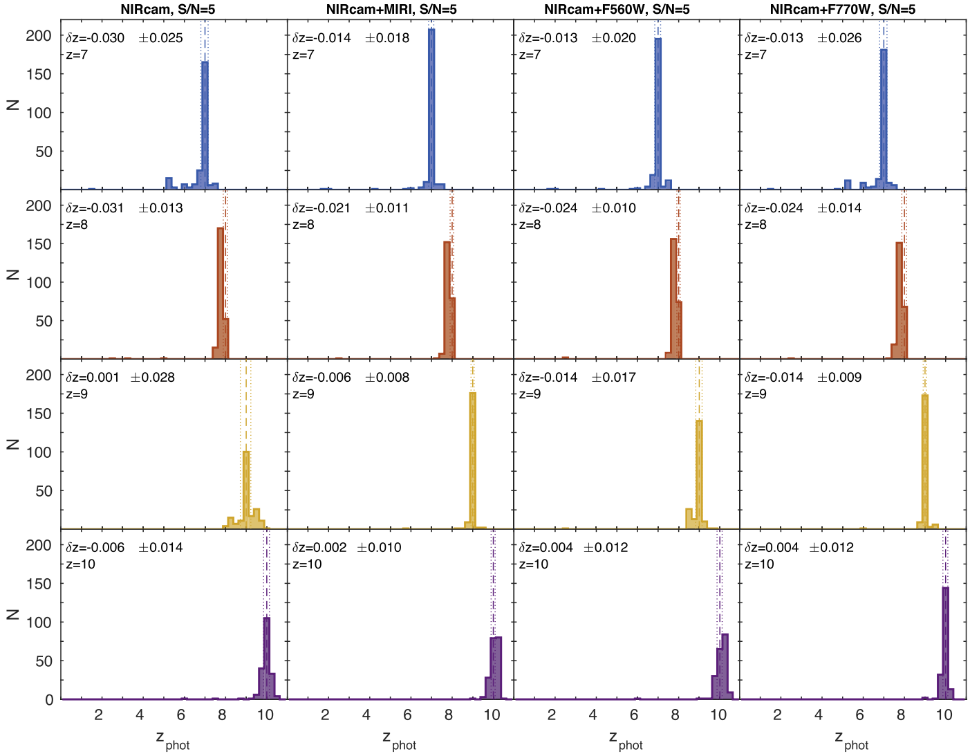
Figure 13. Same as Figure 12, but for (F150W) S/N = 5.
