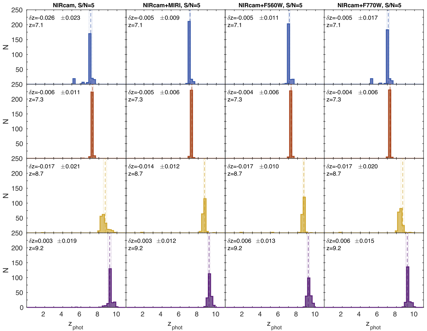
Figure 26. Photometric redshifts obtained for the BC03 simulated galaxies with (F150W) S/N = 5 at different fixed redshifts. From top to bottom: input redshifts z = 7.1, 7.3, 8.7, and 9.2 . Photometric redshifts in each column are obtained with different combinations of bands. From left to right: eight NIRCcam broadbands, eight NIRCcam broadbands, MIRI F560W, and MIRI F770W; eight NIRCcam broadbands and MIRI F560W only; eight NIRCcam broadbands and MIRI F770W only. The vertical lines indicate the 3\sigma interval around the mean normalized redshift difference. On the top left of each panel we quote the mean of (z_{\text{phot}} - z_{\text{input}})/(1 + z_{\text{input}}) and the rms of |z_{\text{phot}} - z_{\text{input}}|/(1 + z_{\text{input}}) .
