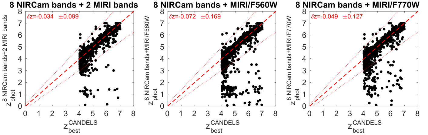
Figure 10. Our derived photometric redshifts vs. CANDELS consensus photometric redshifts for galaxies in sample 2. Left: photometric redshifts obtained with eight NIRCcam broadband and MIRI F560W and F770W. Middle: photometric redshifts obtained with eight NIRCcam broadband and MIRI F560W only. Right: photometric redshifts obtained with eight NIRCcam broadband and MIRI F770W only. The dotted lines in each panel delimit the 3\sigma limit of the |z_{\text{phot}} - z_{\text{fiduc.}}|/(1 + z_{\text{fiduc.}}) distribution, with \sigma = 0.065 , which is the minimum value of \sigma that we get for sample 2 with all the considered filter combinations.
