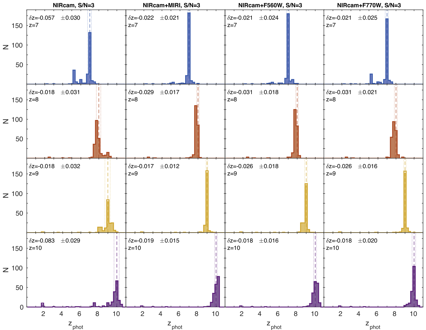
Figure 15. Same as Figure 12, but for (F150W) S/N = 3 .
