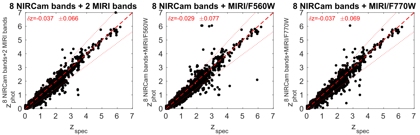
Figure 7. Photometric vs. spectroscopic redshifts for galaxies in sample 1. Left: photometric redshifts obtained with eight NIRCam broadbands and MIRI F560W and F770W. Middle: photometric redshifts obtained with eight NIRCam broadbands and MIRI F560W only. Right: photometric redshift obtained with eight NIRCam broadbands and MIRI F770W only. The dotted lines in each panel delimit the 3\sigma limit of the |z_{\text{phot}} - z_{\text{spec}}|/(1 + z_{\text{spec}}) distribution, with \sigma = 0.058 , which is the minimum value of \sigma that we get for sample 1 with all the considered filter combinations.
