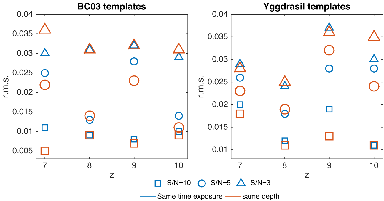
Figure 27. Redshifts vs. rms values of |z_{\text{phot}} - z_{\text{input}}|/(1 + z_{\text{input}}) derived with the NIRCcam broadbands considering the same integration time (blue symbols) or the same observational depth (red symbols). Different symbols correspond to different S/N values: S/N = 10 (squares), 5 (circles), and 3 (triangles). Left: BC03 templates; right: Yggdrasil templates.
