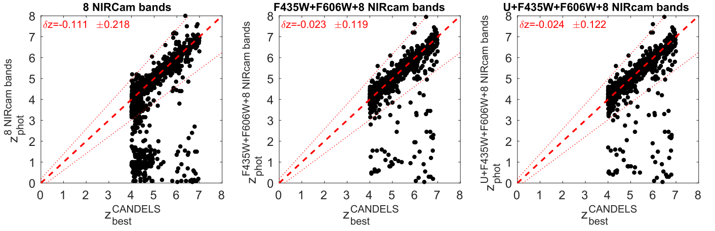
Figure 9. Our derived photometric redshifts vs. CANDELS consensus photometric redshifts for galaxies in sample 2. Left: photometric redshifts obtained with eight NIRCcam broadband. Middle: photometric redshifts obtained with HST F435W and F606W and eight NIRCcam broadband. Right: photometric redshifts obtained with the same bands as in the middle panel plus the VLT U band. The dotted lines in each panel delimit the 3\sigma limit of the |z_{\text{phot}} - z_{\text{fiduc.}}|/(1 + z_{\text{fiduc.}}) distribution, with \sigma = 0.065 , which is the minimum value of \sigma that we get for sample 2 with all the considered filter combinations.
