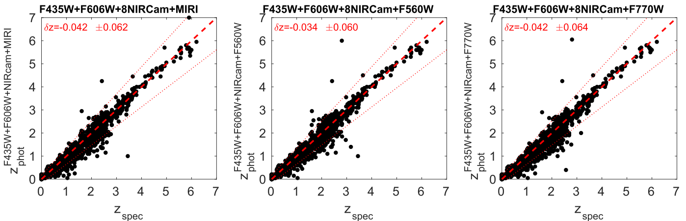
Figure 8. Photometric vs. spectroscopic redshifts for galaxies in sample 1. Left: photometric redshifts obtained with HST F435W and F606W, eight NIRCam broadbands, and MIRI F560W and F770W. Middle: photometric redshifts obtained with HST F435W and F606W, eight NIRCam broadbands, and MIRI F560W. Right: photometric redshifts obtained with HST F435W and F606W, eight NIRCam broadbands, and MIRI F770W. The dotted lines in each panel delimit the 3\sigma limit of the |z_{\text{phot}} - z_{\text{spec}}|/(1 + z_{\text{spec}}) distribution, with \sigma = 0.058 , which is the minimum value of \sigma that we get for sample 1 with all the considered filter combinations.
