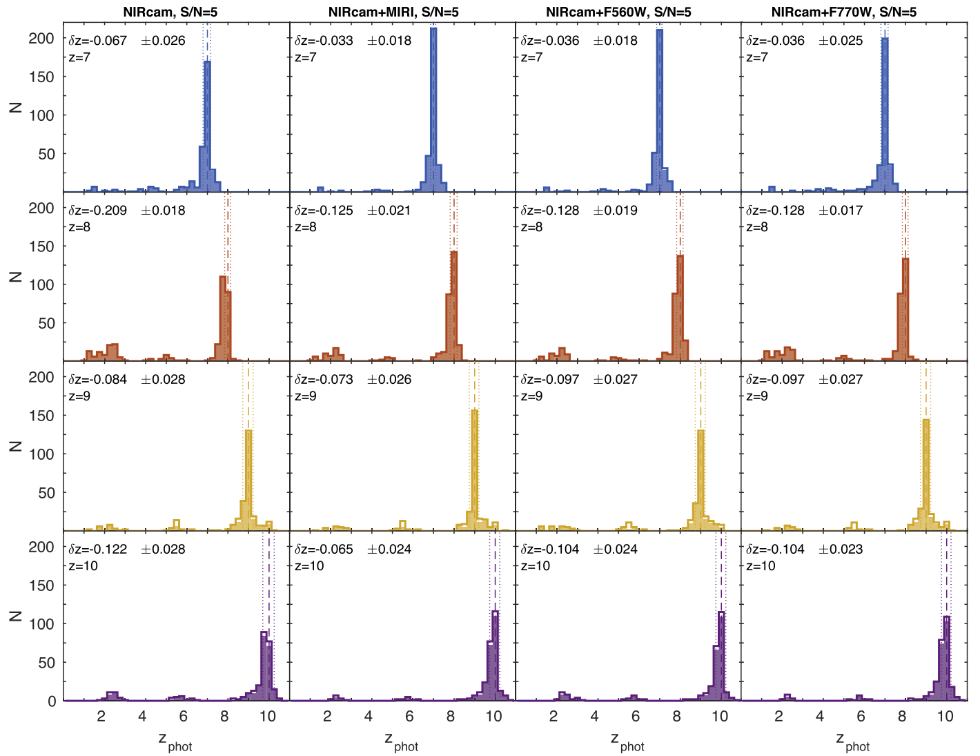
Figure 18. Same as Figure 17, but for S/N = 5 . The shaded area within each histogram corresponds to objects with more than four detections in total in the NIRCcam and MIRI bands, while open areas correspond to sources with less than four band detections.
