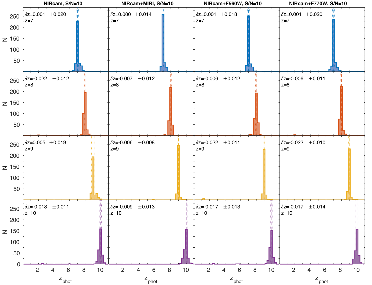
Figure 17. Photometric redshifts for the sample of Yggdrasil simulated galaxies with S/N = 10 . From top to bottom: redshifts z = 7-10 . Photometric redshifts in each column are obtained with different band combinations. From left to right: eight NIRCам broadbands; eight NIRCам broadbands and MIRI F560W, F770W; eight NIRCам broadbands and MIRI F560W only; eight NIRCам broadbands and MIRI F770W only. Each row corresponds to one of the four specific input redshifts. The vertical lines indicate the 3\sigma interval around the mean normalized redshift difference.
