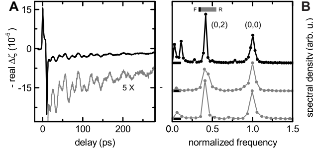
Figure 4.7: (A) Delay scan of a single gold nanoparticle. The oscillation pattern shows a complex modulation. The tail of the trace is also shown 5 \times enlarged. (B) Power spectra of this particle's oscillation (top spectrum) and of two other particles. Frequencies and amplitudes are normalized to those of the (0,0) mode (The absolute frequencies were 67 GHz, 59 GHz, 63 GHz, from top to bottom). The low frequency peak (top spectrum: 28 GHz) lies between calculated frequencies of the (0,2) mode for free boundary (F, thick line on bar) and for rigid boundary (R, end of bar). The ratio of its frequency to that of the breathing mode is constant.
