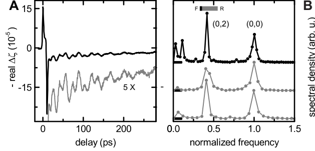
Figure 4.7: (A) Delay scan of a single gold nanoparticle. The oscillation pattern shows a complex modulation. The tail of the trace is also shown 5\times enlarged. (B) Power spectra of this particle's oscillation (top spectrum) and of two other particles. Frequencies and amplitudes are normalized to those of the (0,0) mode (The absolute frequencies were 67 GHz, 59 GHz, 63 GHz, from top to bottom). The low frequency peak (top spectrum: 28 GHz) lies between calculated frequencies of the (0,2) mode for free boundary (F, thick line on bar) and for rigid boundary (R, end of bar). The ratio of its frequency to that of the breathing mode is constant.
