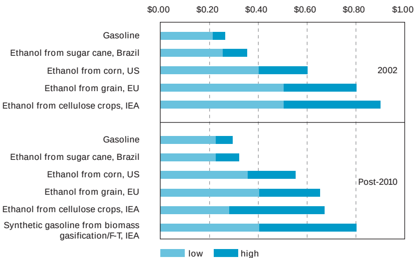
Figure 2 Cost ranges for current and future ethanol production (US dollars per gasoline-equivalent litre)
