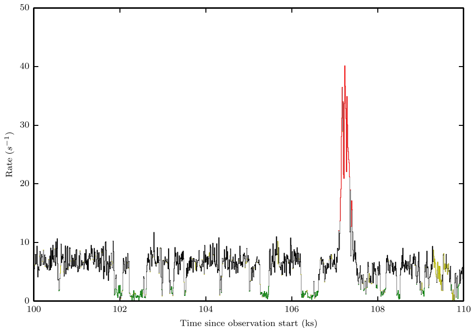
Figure 3. Short section of the combined XMM-Newton light-curve, showing the low (green), high (black), and flare (red) modes. Times at which the mode is indeterminate are marked in gray, and times excluded from pulsation searching because of background flaring are marked in yellow. See Figure 4 for how the thresholds were set, and Figure 7 for the whole light curve.
