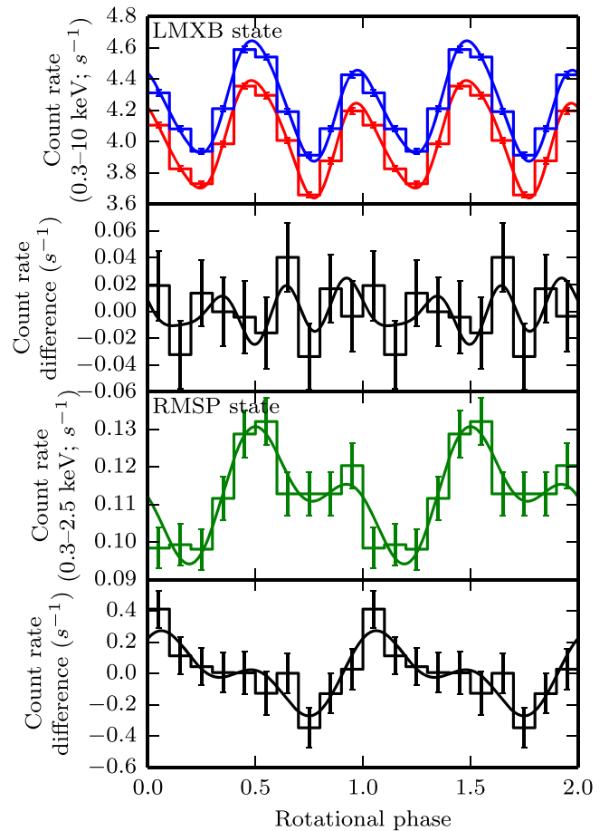
Figure 2. Top panel: the LMXB-state pulse profiles computed from the 2013 November (blue, top) and 2014 June (red, bottom) observations, when the radio pulsar was unobservable. Two rotational cycles are shown for clarity, with both a histogram and a multiple-sinusoid representation (see Appendix A for details). The 2014 November observation has rms amplitude 0.236(6) \text{ s}^{-1} (5.58(13)% modulation) and the 2014 June observation has rms amplitude 0.233(6) \text{ s}^{-1} (5.81(14)%). Second panel: the difference between the scaled LMXB-state profiles. Third panel: the X-ray pulse profile observed during the 2008 November observation reported in Archibald et al. (2010), during which PSR J1023+0038 was in the RMSP state (RMS amplitude 0.0099(18) \text{ s}^{-1} , 8.8(1.6)%). Bottom panel: the difference between the LMXB-state profile (from 2014 June) and a suitably scaled version of that observed during the RMSP state (in 2008 November).
