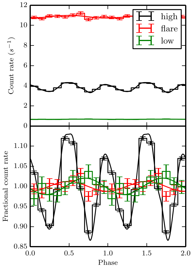
Figure 6. X-ray pulse profiles during the low, high, and flare modes. Each contains background-subtracted combined data from both 2013 November and 2014 June observations. The top panel shows all three normalized by count rate, while the bottom panel shows all three normalized to the same mean value. In the low mode, pulsations are not detected: the H test reports a false positive probability of 0.2; a 95% confidence upper limit on the plausible pulsed fraction is about 2.4% (that is, if the pulsed fraction were 2.4% we would obtain a false positive probability smaller than this 95% of the time). This corresponds to a maximum possible pulsed flux in the low mode of 0.016 \text{ s}^{-1} . In the high mode, the pulsed flux (fraction) is 0.311(5) \text{ s}^{-1} (8.13(14)%). In the flare mode we also do not detect pulsations with a false positive probability of 0.2, giving an upper limit on the pulsed fraction of 1.4% and the pulsed flux of 0.15 \text{ s}^{-1} ; note that this 95% upper limit on the pulsed flux is less than the pulsed flux during the high mode.
