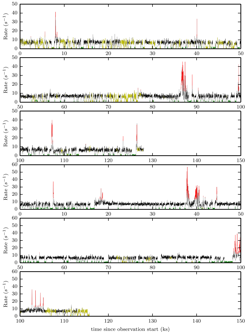
Figure 5. Combined X-ray light curve showing classification of times into low, high, flare, ambiguous, or background flaring. This light curve is formed using exposure-corrected and background-subtracted data from the pn and both MOS cameras in 10 s time bins. Regions marked in green are classified as low-mode, black as high-mode, and red as flares; the gray regions were treated as ambiguous, and the yellow regions suffered from background flaring, and neither were used in pulsation searches. The top three panels of this light curve are from the 2013 November observation, while the bottom three are from the 2014 June observation.
