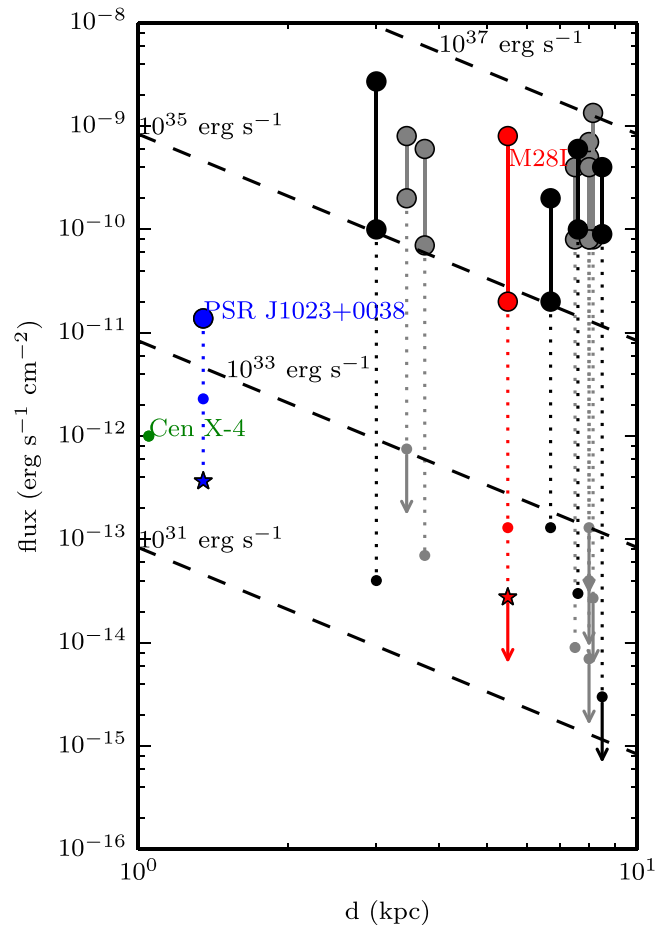
Figure 7. Approximate X-ray fluxes of AMXPs. Large circles connected by solid lines indicate the range of fluxes at which coherent X-ray pulsations have been detected, while dotted lines and small circles indicate the range of quiescent flux levels (arrows indicate where only an upper limit on quiescent flux is available). Stars indicate X-ray fluxes during a RMSP state. The horizontal axis is distance, generally the largest uncertainty, and the dashed diagonal lines show constant luminosities. Marked in red is the transition system PSR J1824–2452I (also called M281), and in blue is PSR J1023+0038 (in both cases the distances are well known). For PSR J1023+0038, the large circle shows the high-state flux (where pulsations were detected) and the small circle shows low-state flux (where no pulsations were detected). Cen X-4 is marked in green. AMXPs with relatively good distance estimates are marked in black, whereas those where the distance is more uncertain are marked in gray. For details and references see Table 1.
