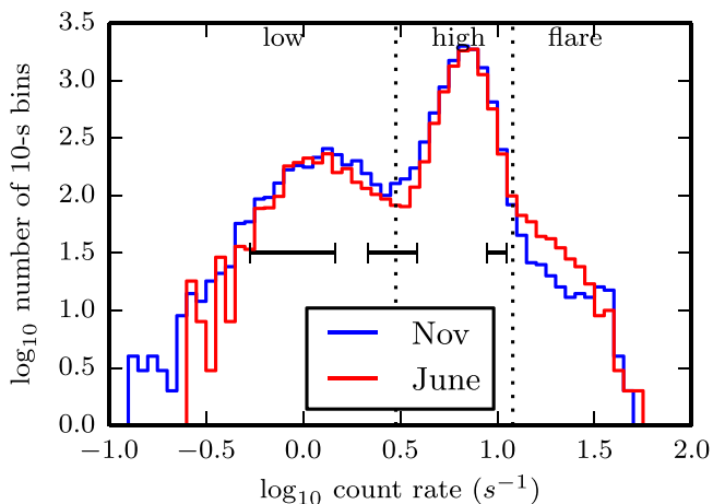
Figure 4. Distribution of fluxes in the 2013 November and 2014 June observations. All pn and MOS photons from both observations were combined to form an exposure-corrected light curve with 10 s time bins, and histograms of the resulting count rates are plotted. Horizontal error bars show the horizontal smearing due to Poisson noise in the light curve bins. Vertical dotted lines show the cuts we chose between low, high, and flare modes.
