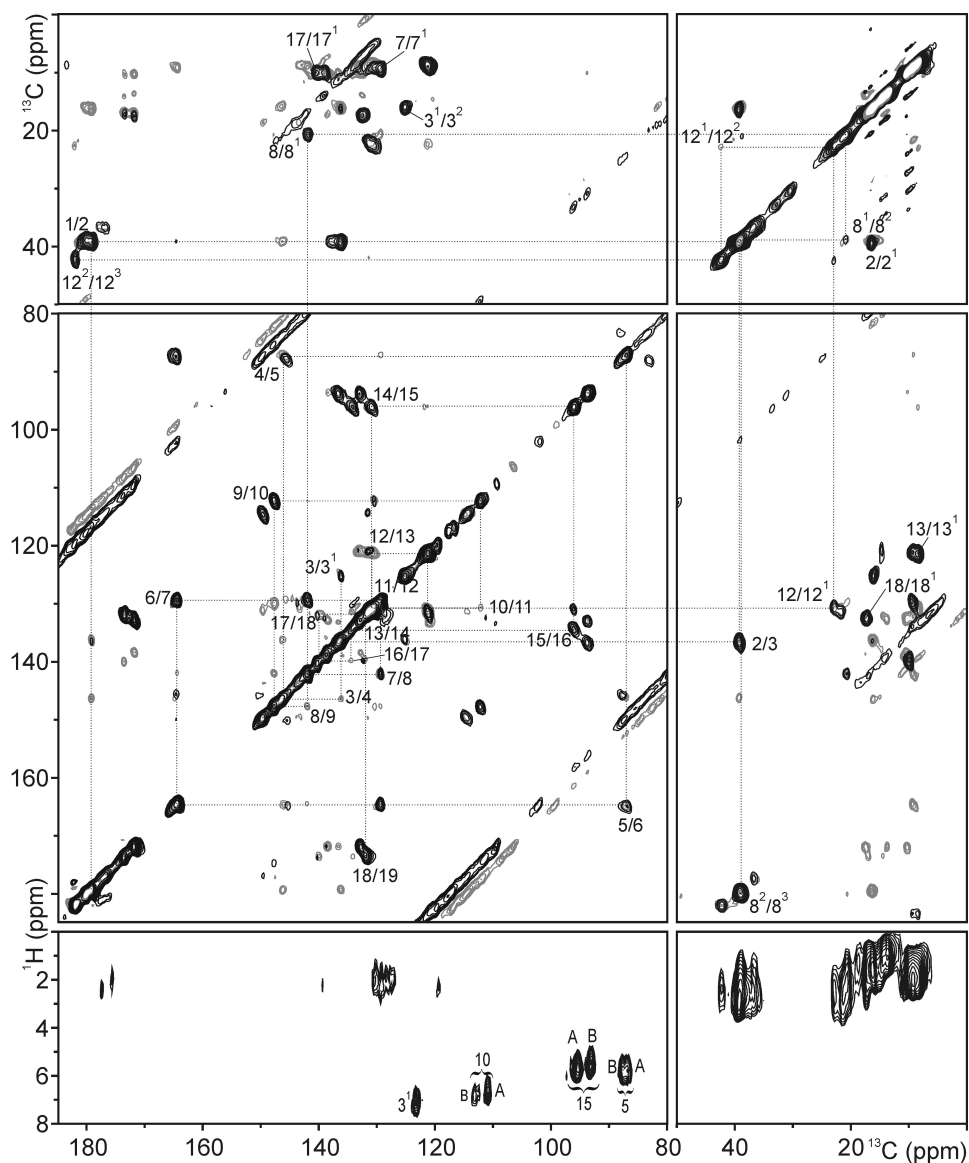
Figure 2.3: The upper panels show the contour plots of ^{13}\text{C} - ^{13}\text{C} RFDR MAS NMR spectrum of u\text{-}[^{13}\text{C}, ^{15}\text{N}]\text{-PCB} recorded in a field of 17.6 T using spinning frequencies of 11800 Hz (black) and 12500 Hz (grey), and mixing times of 1.8 ms and 3.2 ms, respectively. The lower panels represent the contour plot of the ^1\text{H} - ^{13}\text{C} FSLG MAS NMR dipolar correlation spectrum at a spinning frequency of 11800 Hz.
