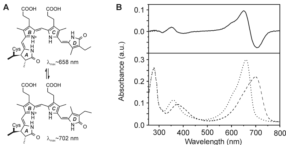
Figure 1.2: Photoconversion of cyanobacterial phytochrome 1 (Cph1). (A) Structure of the phycocyanobilin chromophore with ZZZssa and ZZEssa geometries as assumed in the Pr and Pfr states, respectively. (B) Absorption spectrum of Cph1 in the Pr (dotted line), Pfr (dashed line) and Pr-Pfr difference spectrum (full line).
