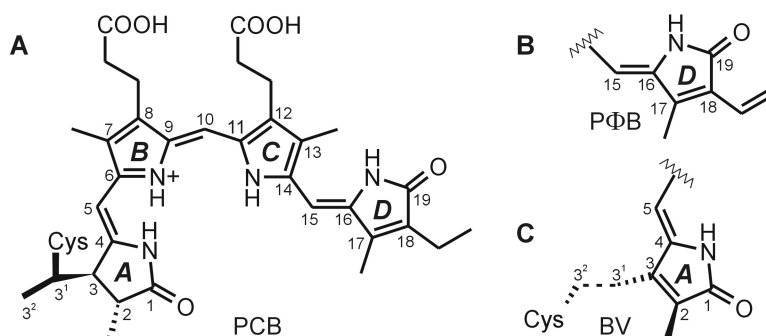
Figure 1.4: Structure of the phycocyanobilin (PCB) in the ZZZssa geometry ( A ). Ring D of phytochromobilin (PΦB, B ) and ring A of biliverdin (BV, C ) are represented. The remainder of these molecules is identical to PCB.
