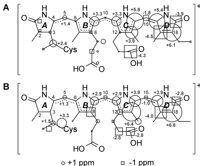
Figure 3.4: Changes in ^{13}\text{C} chemical shifts of the u- [^{13}\text{C}, ^{15}\text{N}] -PCB chromophore in Cph1Δ2 (A) and phyA65 (B). The Pr state is taken as reference and the size of the circles and squares refers to the difference in ^{13}\text{C} chemical shift in the Pfr state. The carbons showing two resonances are labeled with two symbols. The positive charge due to the protonation of the ring B nitrogen is thought to be delocalized mainly over rings B and C, and the non planarity of the C14–C15 single bond breaks the conjugation with ring D.
