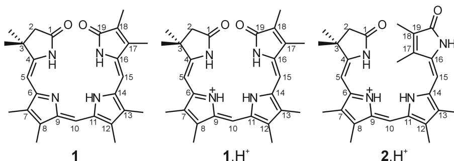
Figure 5.1: Structures of the 1 and 1.H + model compounds in the ZZZsss geometry. 2.H + is the E -diastereoisomer of 1.H + in its ZZEsss geometry. The extent of positive charge is resrepresented on ring B , as assumed in [103].
