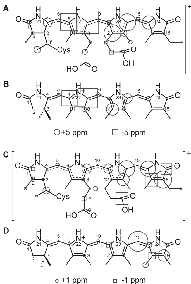
Figure 5.2: The upper part (A and B) shows the change in ^{13}\text{C} chemical shifts resulting from the assembly of PCB into Cph1Δ2 (PCB \rightarrow Pr, A) and upon protonation of 1 ( 1 \rightarrow 1.H^+ , B). The lower part (C and D) represents the changes in ^{13}\text{C} chemical shifts accompanying Pr \rightarrow Pfr conversion (C) and the difference in ^{13}\text{C} shifts between the models compound of the 1.H^+ and 2.H^+ (D). The free PCB (A form), 1, Pr and 1.H^+ are taken as reference in A, B, C and D, respectively. The upshifts of the ^{13}\text{C} resonances of C3 and C3 1 due to the formation of the thioether linkage with Cys-259 (82.8 and 77.4, respectively) are not represented in A.
