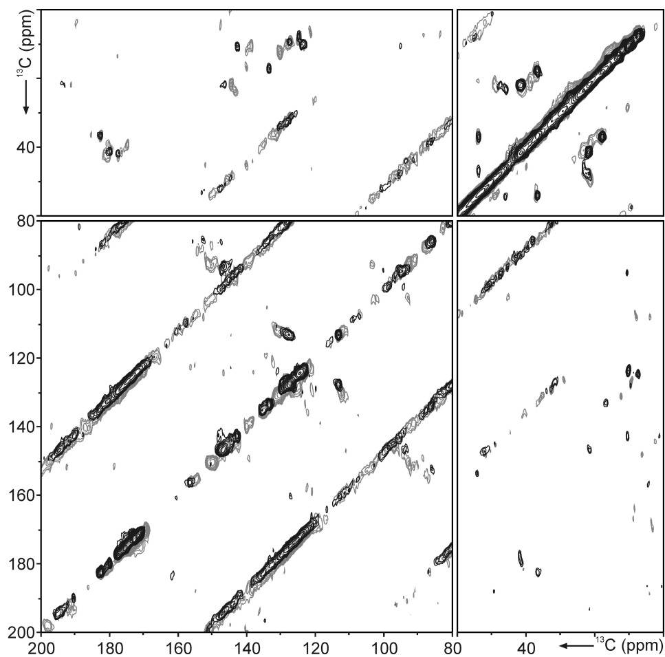
Figure B.5: Contour plot of the 2D ^{13}\text{C} - ^{13}\text{C} DARR NMR spectra of u\text{-}[^{13}\text{C}, ^{15}\text{N}]\text{-PCB-phyA65} in the Pr (black) and Pfr states (grey). The spectra were recorded with proton mixing times of 5 ms, at 243 K and with a spinning frequency of 9 kHz.
