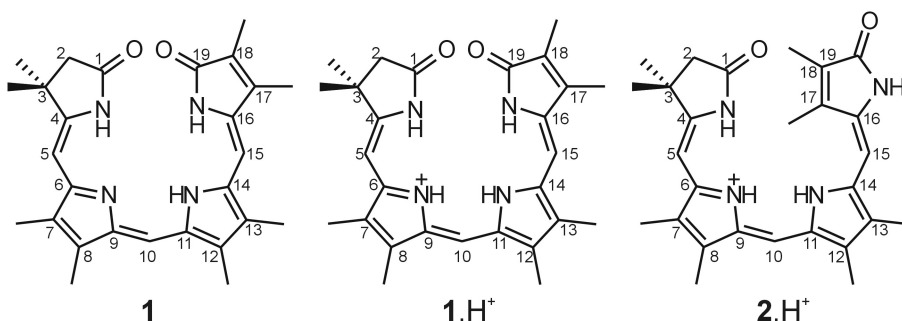
Figure 5.1: Structures of the 1 and 1.H + model compounds in the ZZZ ss geometry. 2.H + is the E -diastereoisomer of 1.H + in its ZZE ss geometry. The extent of positive charge is resrepresented on ring B , as assumed in [103].
