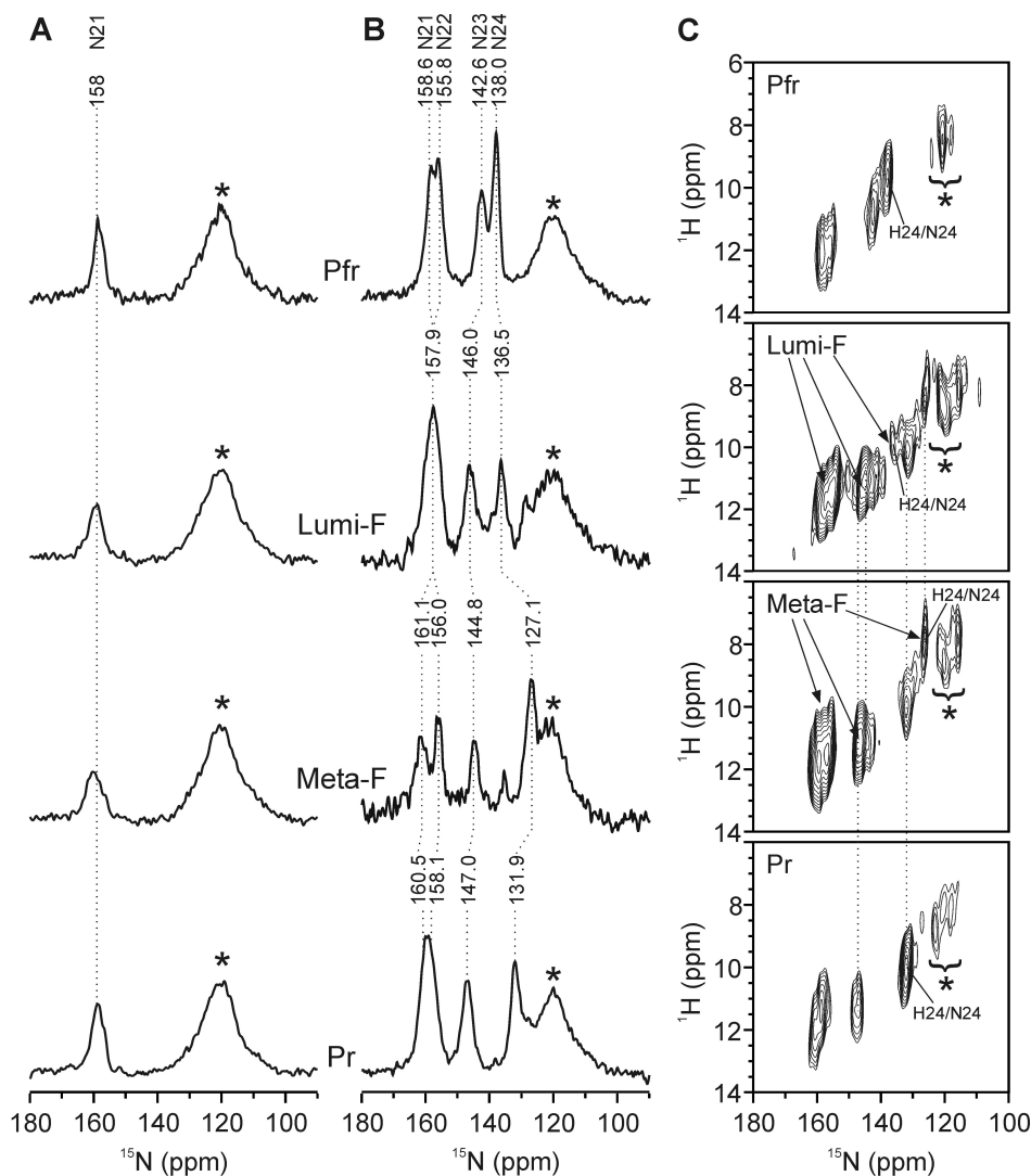
Figure 4.5: 1D ^{15}\text{N} spectra of ^{15}\text{N} 21-PCB-Cph1 \Delta 2 (column A) and ^{15}\text{N} -PCB-Cph1 \Delta 2 (column B) in the Pfr, Lumi-F, Meta-F and Pr states recorded at 17.6 T with a spinning frequency of 8 kHz and at 243 K, 173 K, 203 K, and 243 K, respectively. 2D ^1\text{H} - ^{15}\text{N} FSLG heteronuclear correlation spectra of Pfr, Lumi-F, Meta-F, and Pr (Column C). The spectra of the intermediates were obtained from a Pfr:Pr (1:1) mixture.
