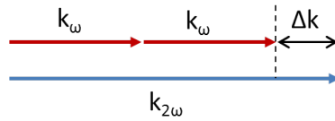
Figure 1.2: The wave-vector mismatch for collinear second harmonic generation as a result of dispersion in the refractive index of the nonlinear material. Note that for most materials the refractive index for blue wavelengths is larger than the refractive index for red wavelengths.
