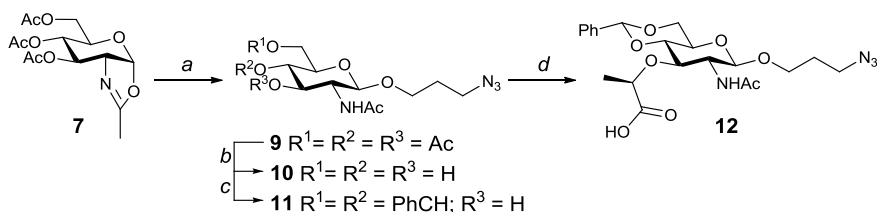
Scheme 1. Synthesis of building block 12 .
