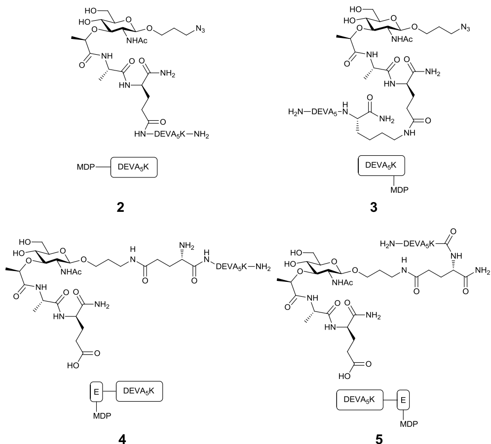
Figure 3. NOD2-L-antigen conjugates 2 – 5 , DEVA 5 K = DEVSGLEQLESIINFELKAAAAAK.
