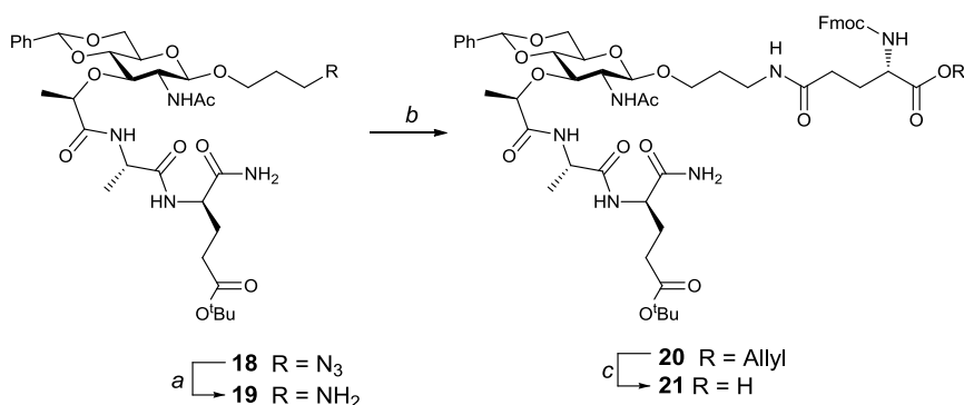
Scheme 3. Synthesis of 21 .
