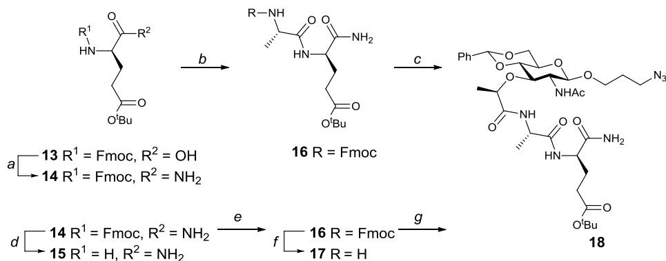
Scheme 2. Synthesis of building block 18 .
