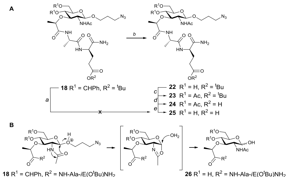
Scheme 4. Synthesis of reference compound 25 .
