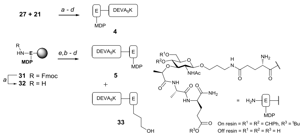
Scheme 6. SPPS of conjugates 4 and 5 .
