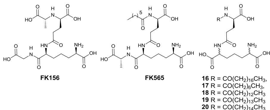
Figure 6. Compounds FK-156, FK-565 and 16 – 20 .
