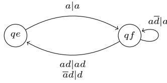
Figure 2.12: Reo Automaton for LossyFIFO1
