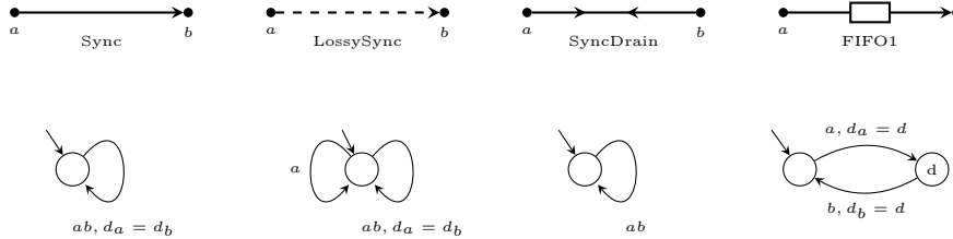
Figure 2.6: Constraint Automata for basic Reo channels of Figure 2.1
