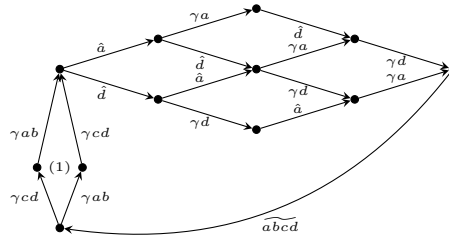
Figure 4.11: Composed IMC for 2sync
