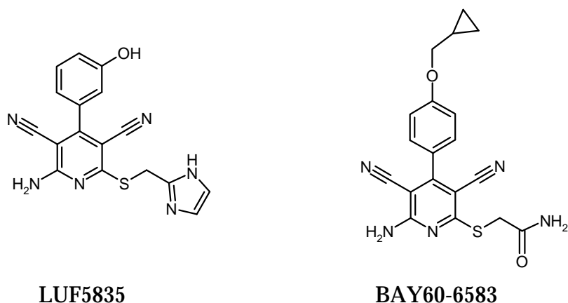
Figure 7. Chemical structure of two non-ribose adenosine A_{2B} receptor agonists: LUF5835 and BAY 60-6583.
