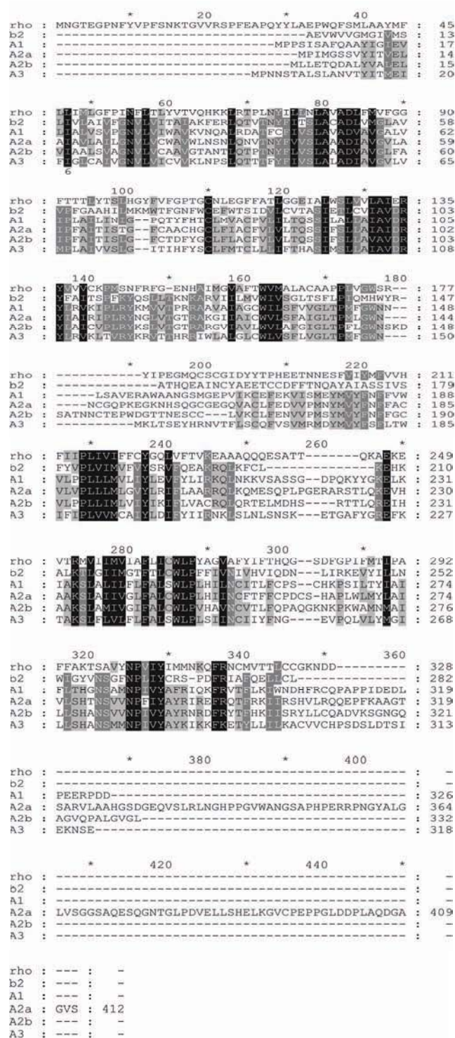
Figure 2. Multiple amino acid sequence alignment of the human adenosine A 1 , A 2A , A 2B , A 3 , human β 2 adrenergic receptors and bovine rhodopsin. Conserved residues are marked in black. Similar residues are marked in grey.
